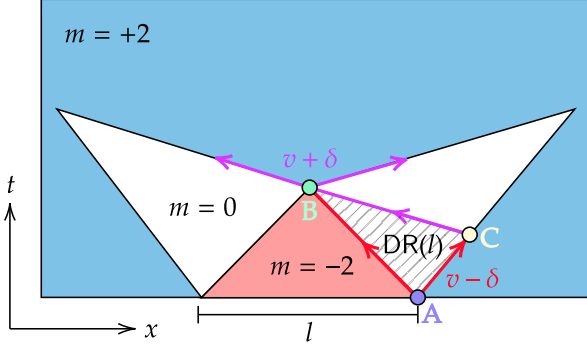
FIG. 2. How a minority domain of size l is eroded under ideal sliding dynamics with v > 2 in the limit \beta J \rightarrow \infty . The white regions have zero magnetization, and are metastable. The red arrows indicate interfaces that move with expected speed v - \delta , and the purple arrows those with speed v + \delta . The danger region DR(l) indicated by the shaded triangle is the spacetime region where spin flips in the metastable zero-magnetization area can propagate to prevent the erosion of the m = -2 (red) part of the initial minority domain.
