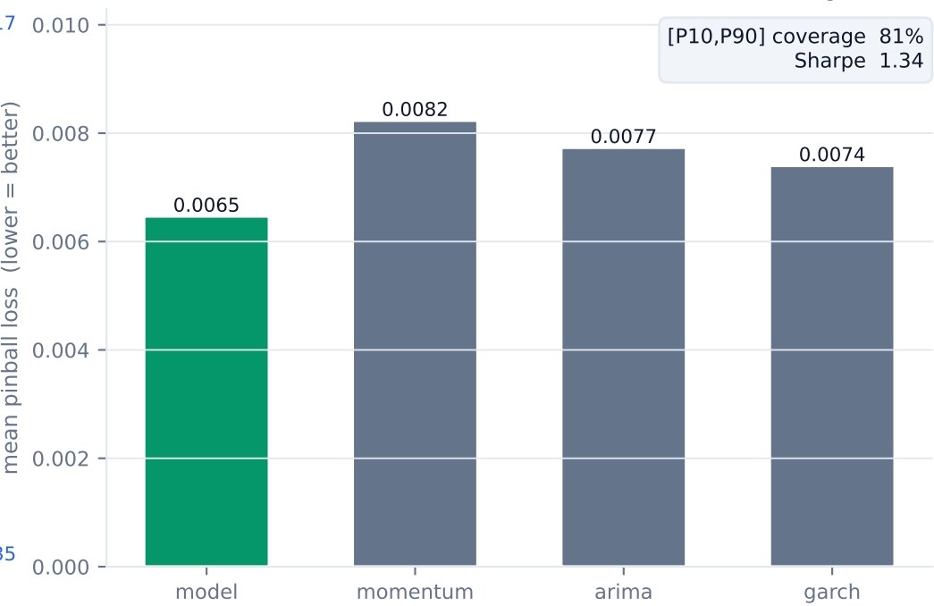
Backtest · 1d horizon · n=248 walk-forward preds
