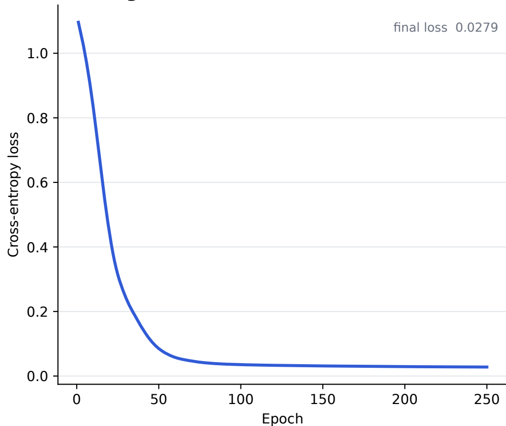
Training loss
