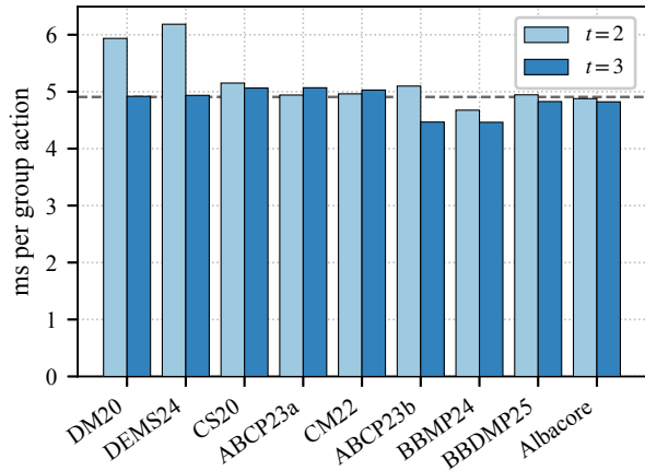
(b) time per counted group action
