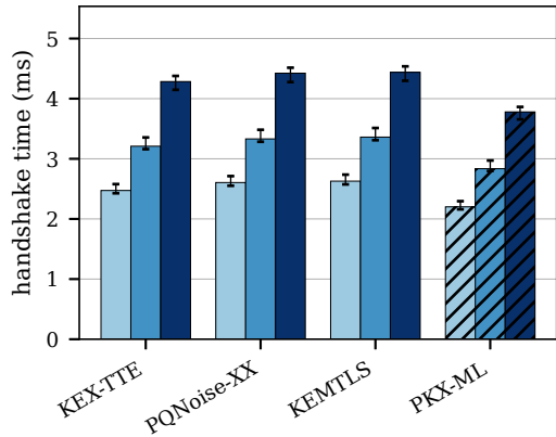
(b) transmitted static keys (XX)
