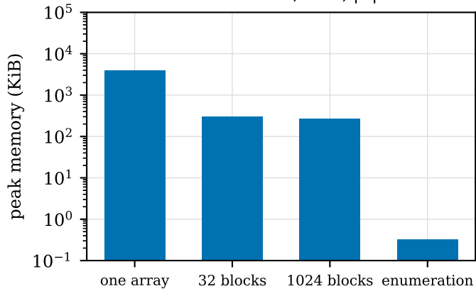
relation collection, t = 4 , |H| = 2^{20}
