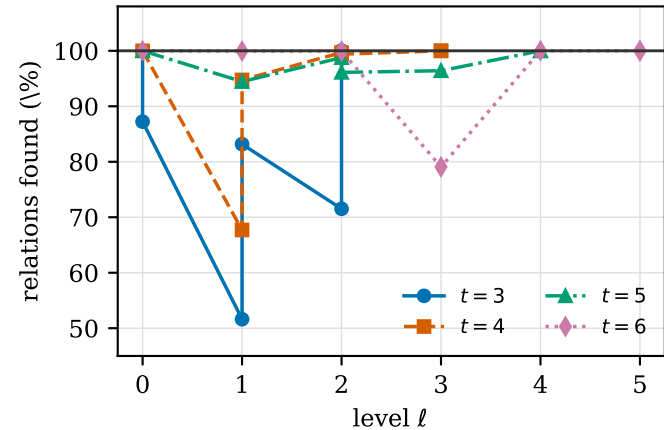
completeness of the transition sieve
