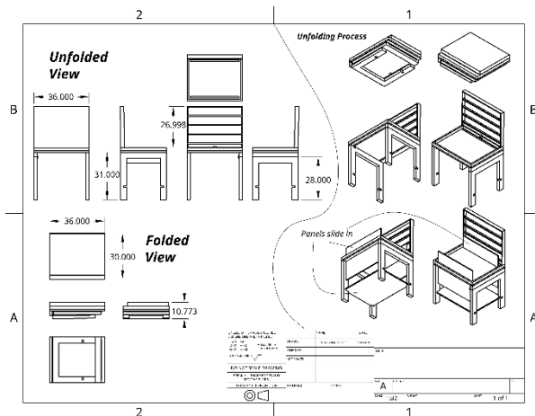
Figure 19: Kiosk Orthographic Drawing
