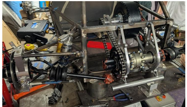
Figure 7: Integrating TSP into rear drive train
