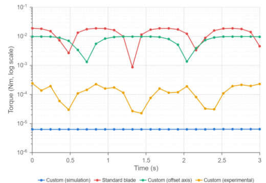
Figure 13: Simulated and measured torque vs. time over average stroke duration (3 s). The custom putter showed markedly lower and more consistent torque than alternatives in simulation; experimental testing confirmed a significant reduction, though smaller than predicted theoretically.
