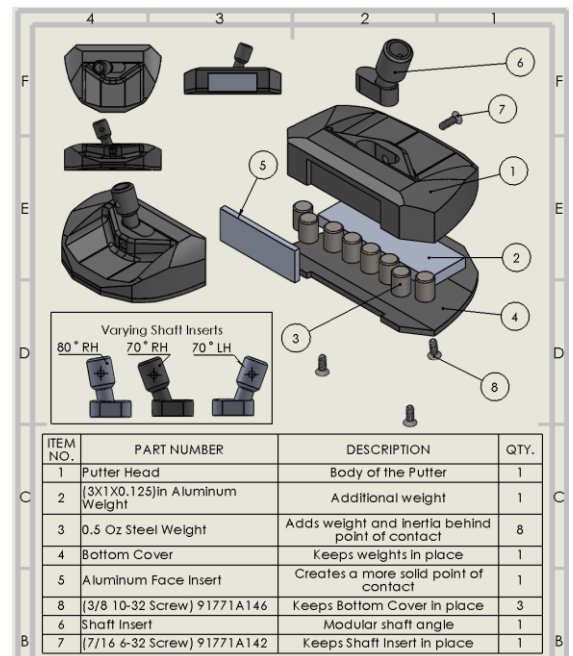
Figure 12: Final Product, Optimal Weight Distribution and sufficient Mass (192g)
