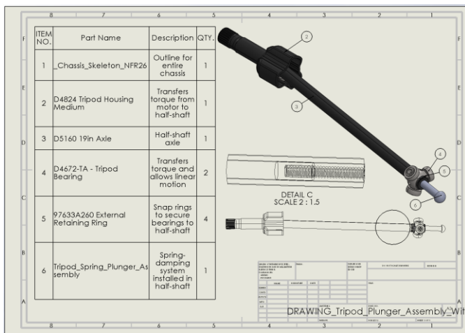
Figure 4: Half Shaft Drawing and BOM, including TSP.
