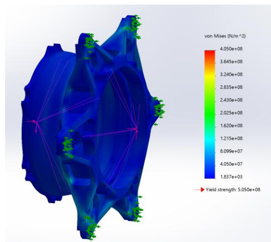
Figure 3: Hubs Outside Cornering FEA Case (Stress)
