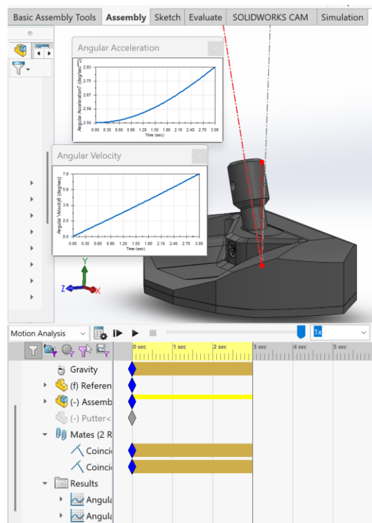
Figure 10: Motion Analysis Simulation
