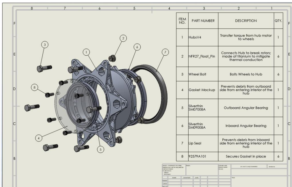
Figure 1: Full Hub Exploded View & BOM
