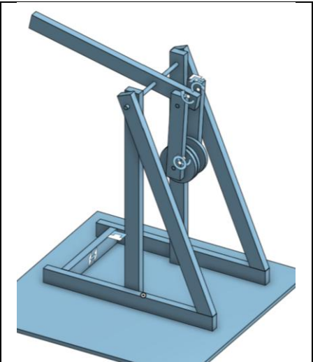
Figure 27: Onshape CAD approximation
