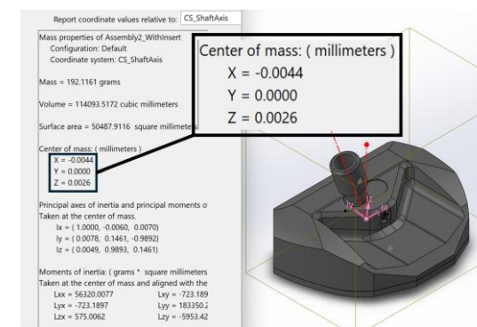
Figure 11: Mass Analysis on Final Product; Results show C.O.M very closely aligned with the shaft axis (~4 microns)
