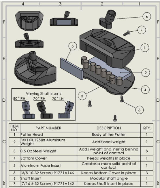
Figure 13: Final Product, Optimal Weight Distribution and sufficient Mass (192g)
