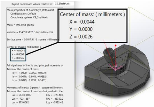
Figure 12: Mass Analysis on Final Product; Results show C.O.M very closely aligned with the shaft axis (~4 microns)
