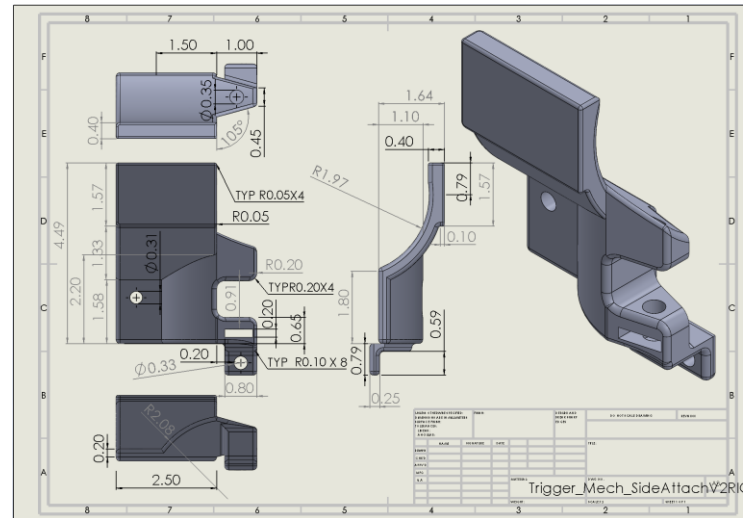
Figure 16: Example of a Fully Dimensioned Part
