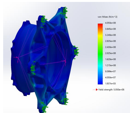
Figure 4: Hubs Outside Cornering FEA Case (Stress)
