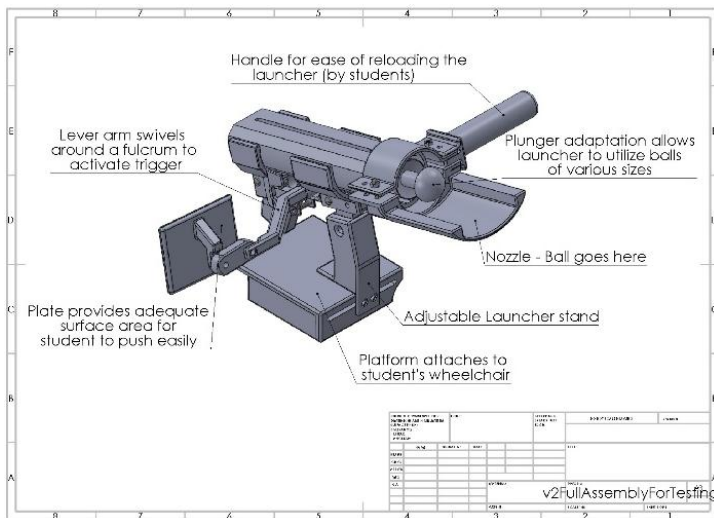
Figure 15: Isometric View and Descriptions
