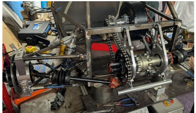
Figure 8: Integrating TSP into rear drive train
