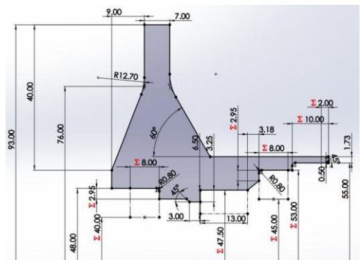
Figure 2: Design Space and Essential Geometry
