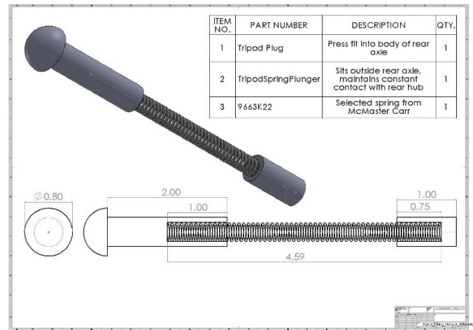
Figure 6: TSP Dimensioned Assembly
