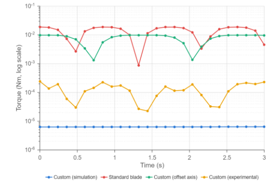
Figure 14: Simulated and measured torque vs. time over average stroke duration (3 s). The custom putter showed markedly lower and more consistent torque than alternatives in simulation; experimental testing confirmed a significant reduction, though smaller than predicted theoretically.
