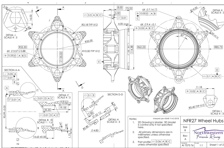
Figure 1: Hubs GD&T Design Drawing
