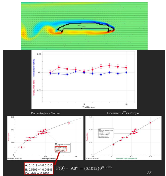
Figure 25: Some Experiment Results
