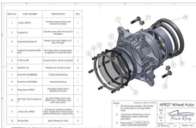
Figure 3: Full Hub Exploded View & BOM
