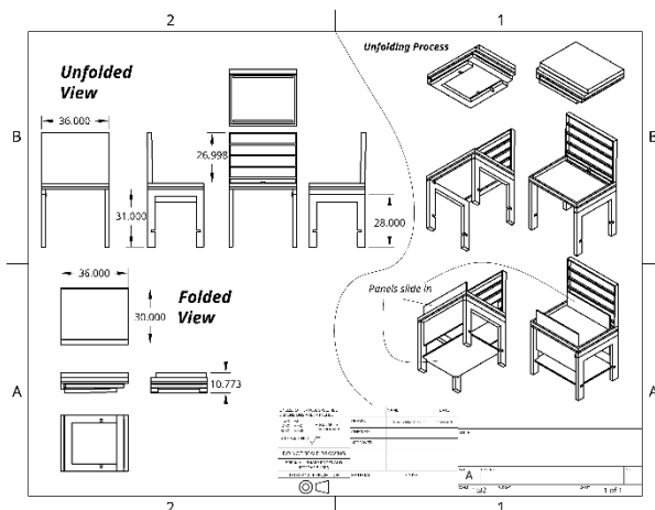
Figure 20: Kiosk Orthographic Drawing
