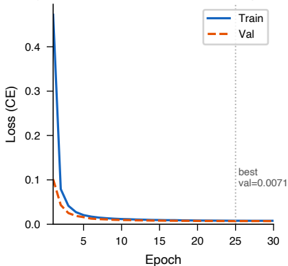
(B) GRU-VAE Fine-tuning (1,401 ChEMBL PPI inhibitors, 30 epochs)
