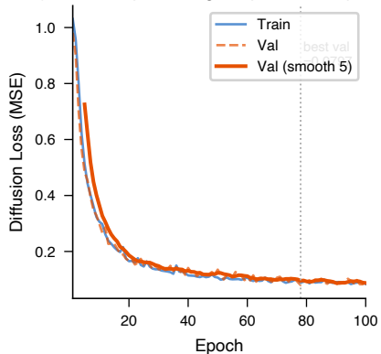
(C) Conditional DDPM Training (MW > 350 pocket-ligand pairs, 100 epochs)
