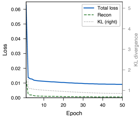
(A) GRU-VAE Pre-training (ZINC 100k, 50 epochs)
