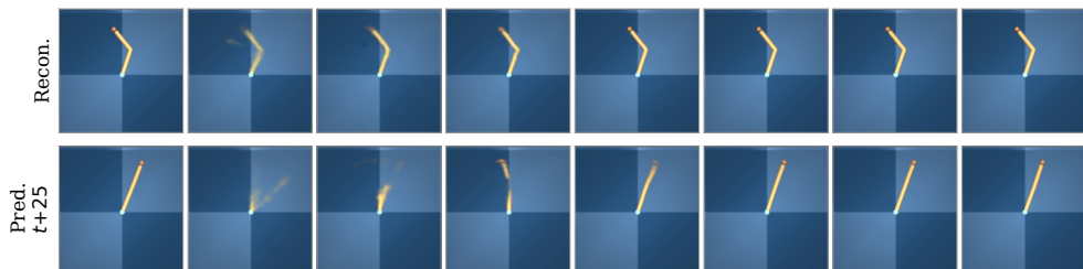
Reacher
