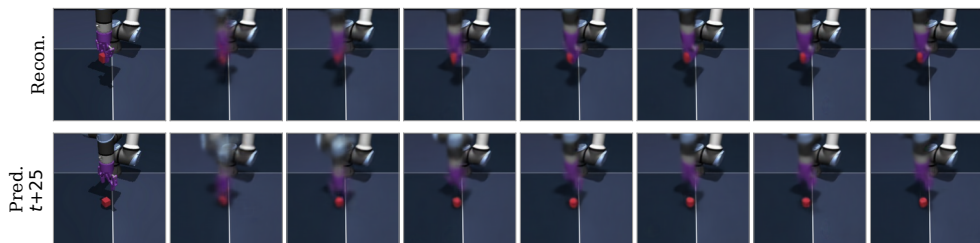
OGBench-Cube
