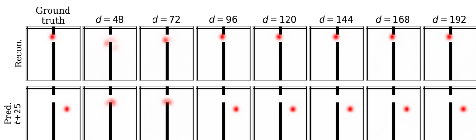
TwoRoom
