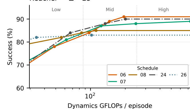
Reacher — \Delta = 25
