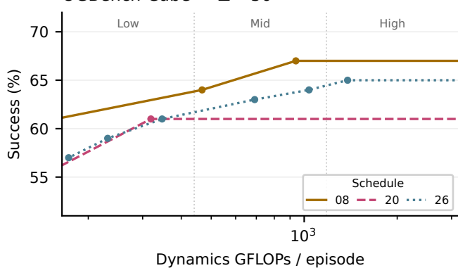
OGBench-Cube — \Delta = 50
