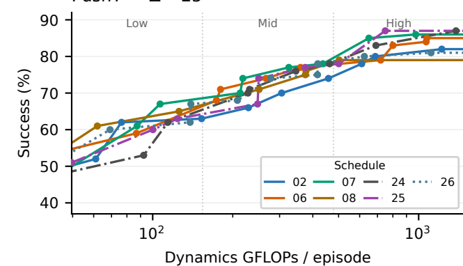
PushT — \Delta = 25
