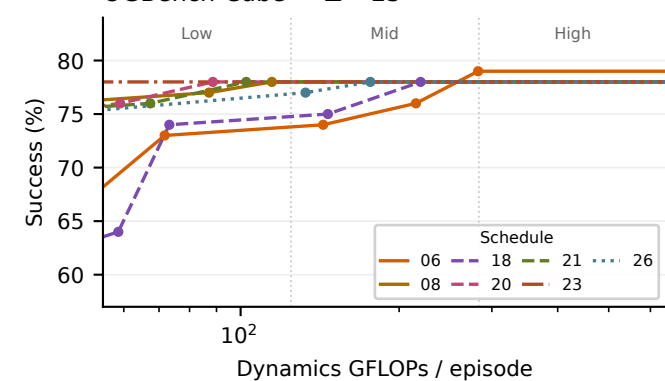
OGBench-Cube — \Delta = 25
