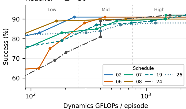
Reacher — \Delta = 50
