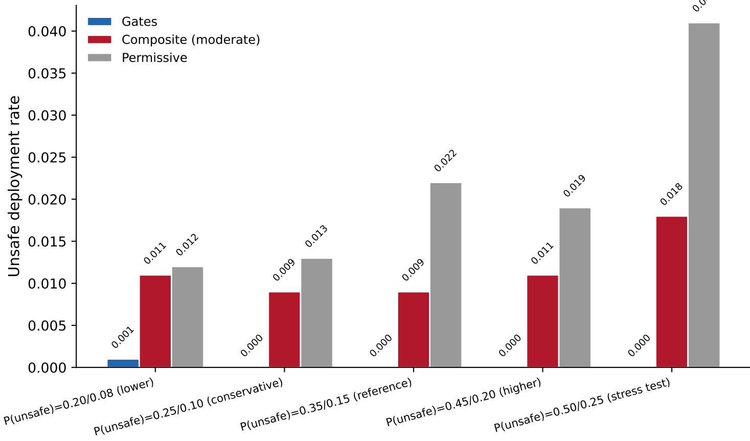
Unsafe Deployment Rate by Unsafe Probability
