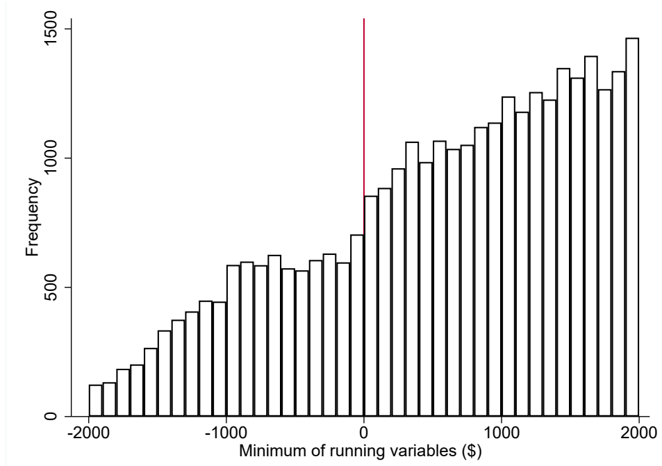
(a) Histogram
