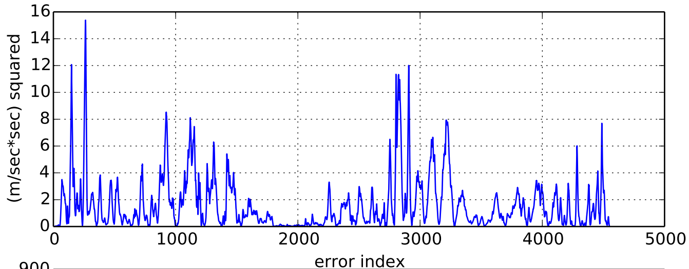
imu0: acceleration error
