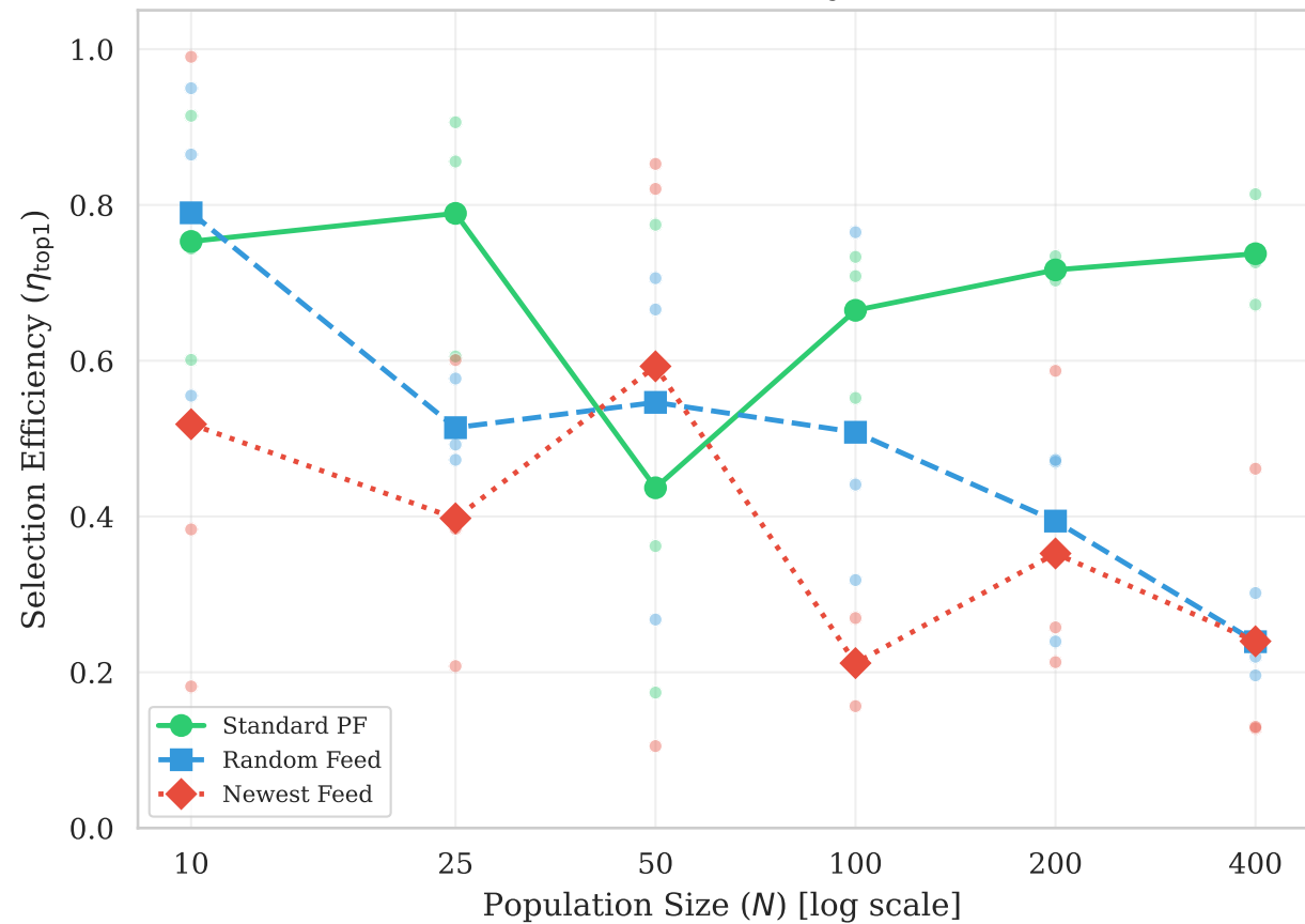
(a) Selection Efficiency vs Scale
