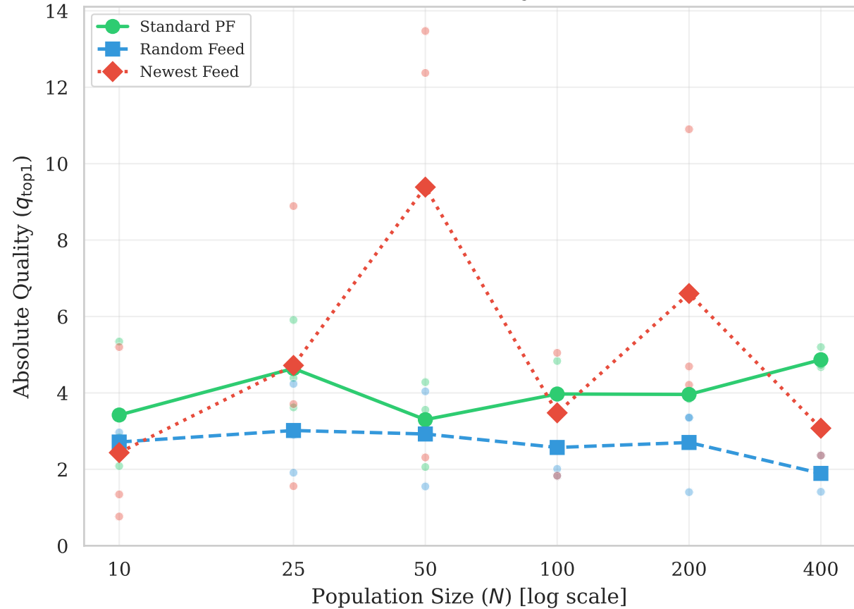
(b) Absolute Quality vs Scale
