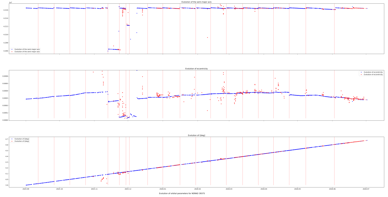
Evolution of orbital parameters for NORAD 28885
