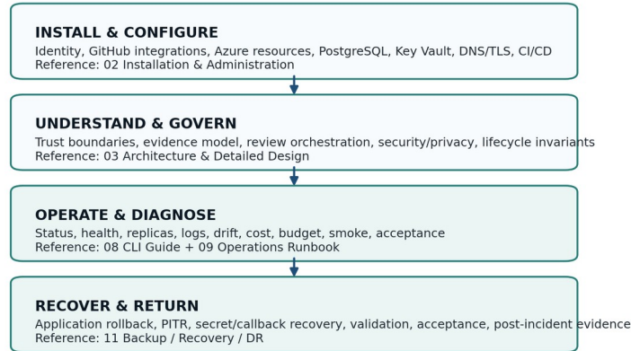
Figure 4. Production responsibility stack. Installation establishes the system; operations and recovery preserve it over time. Historical reference figure; current text governs.
