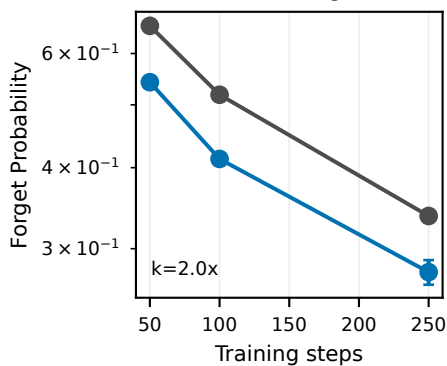
SimNPO / forget10
