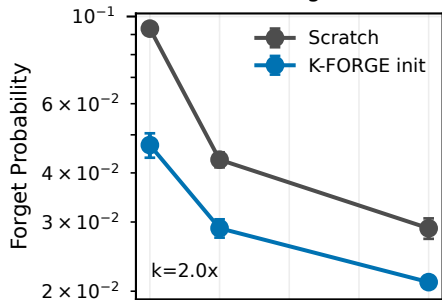
NPO / forget10
