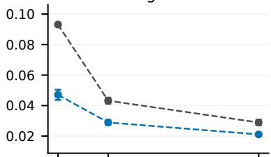
forget10
