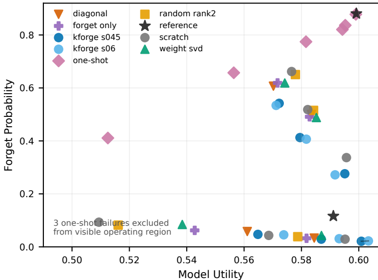
TOFU forget10 corrected Pareto frontier
