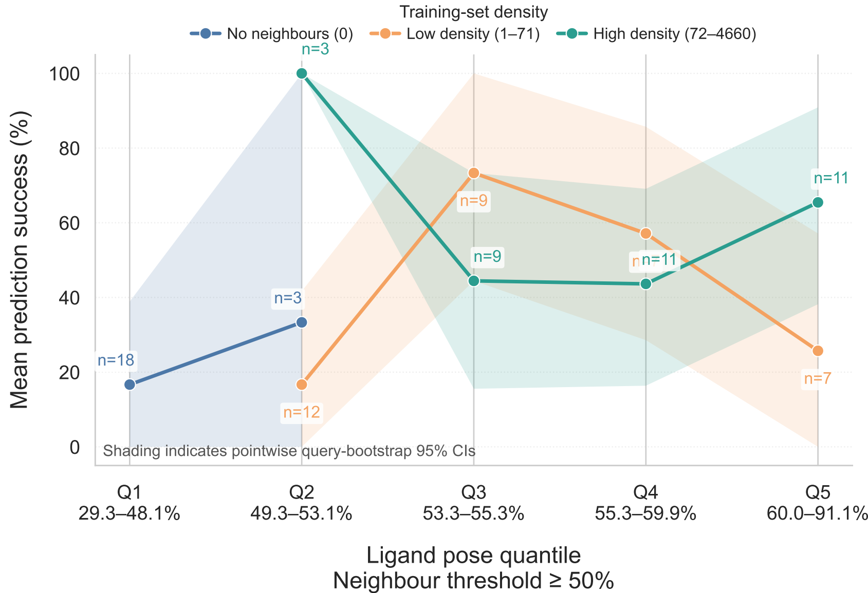
Boltz-1
