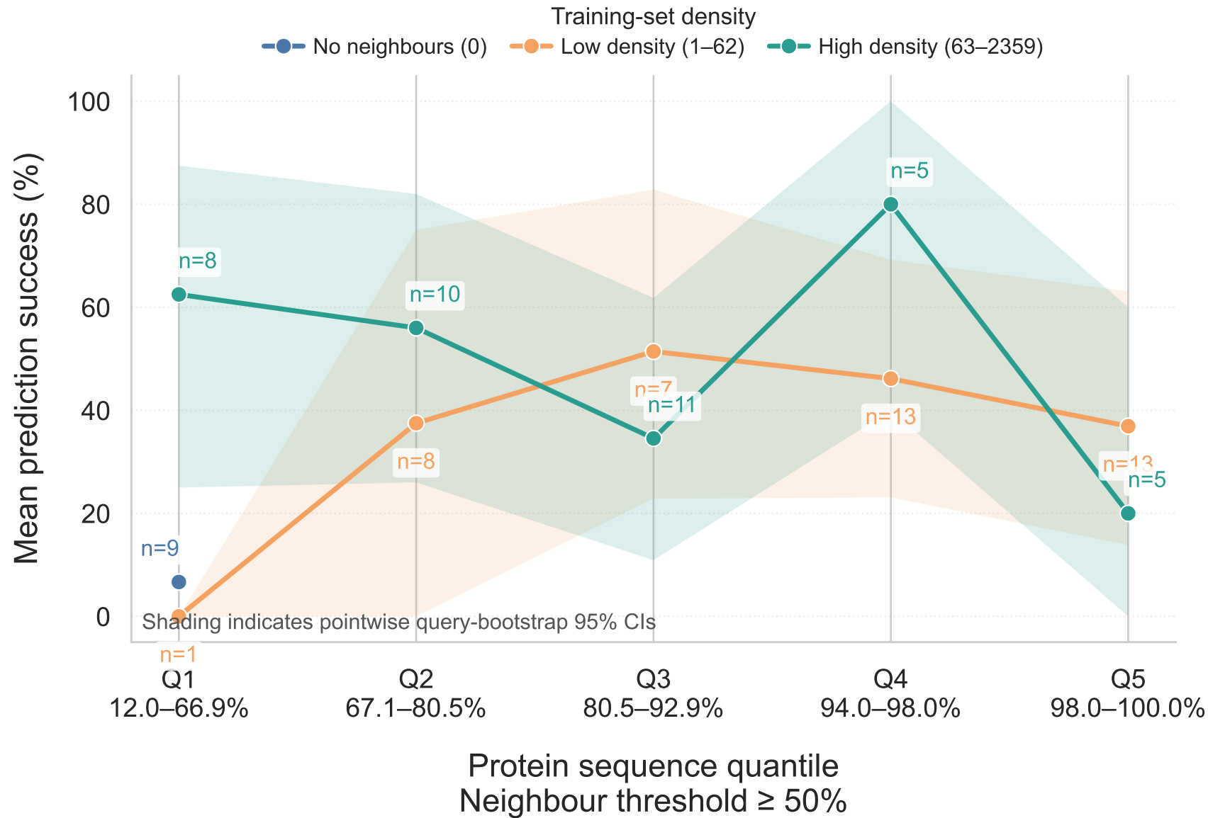
Boltz-1
