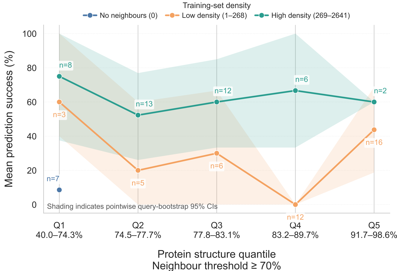
Boltz-1
