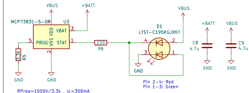
LiPo Charger
