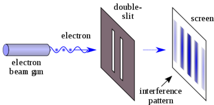
FIGURE 1.9: Double-slit Experiment
