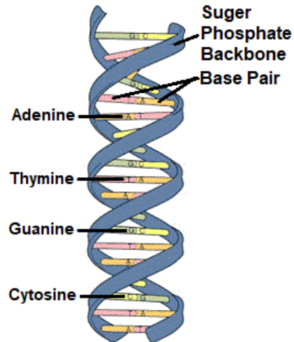
FIGURE 6.6: DNA Double Helix Molecule
