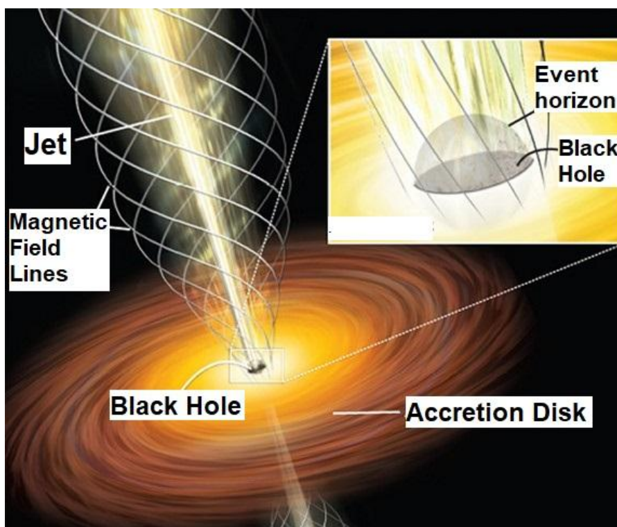
FIGURE 3.26: Column of Magnetic Field
