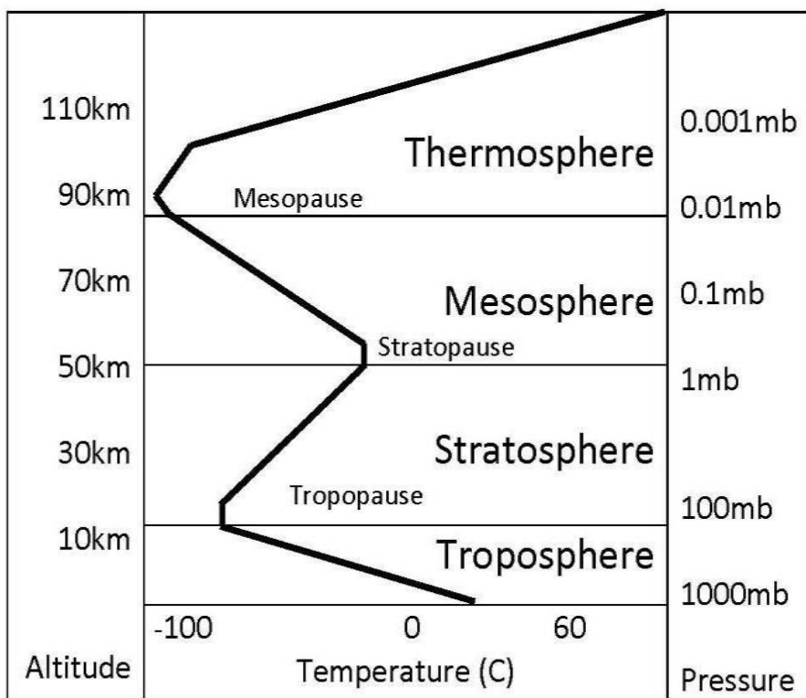
FIGURE 2.5: Temperature Curve
