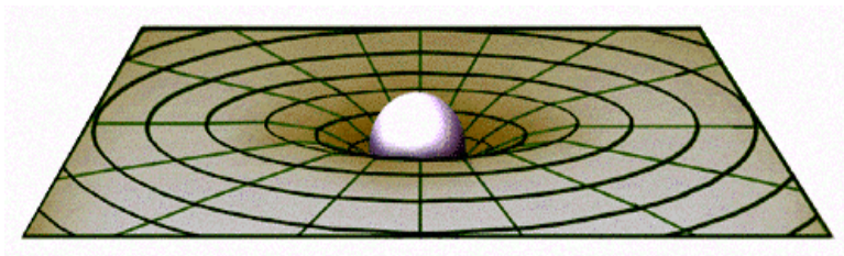
FIGURE 2.17: Curvature of space in two dimensional view
