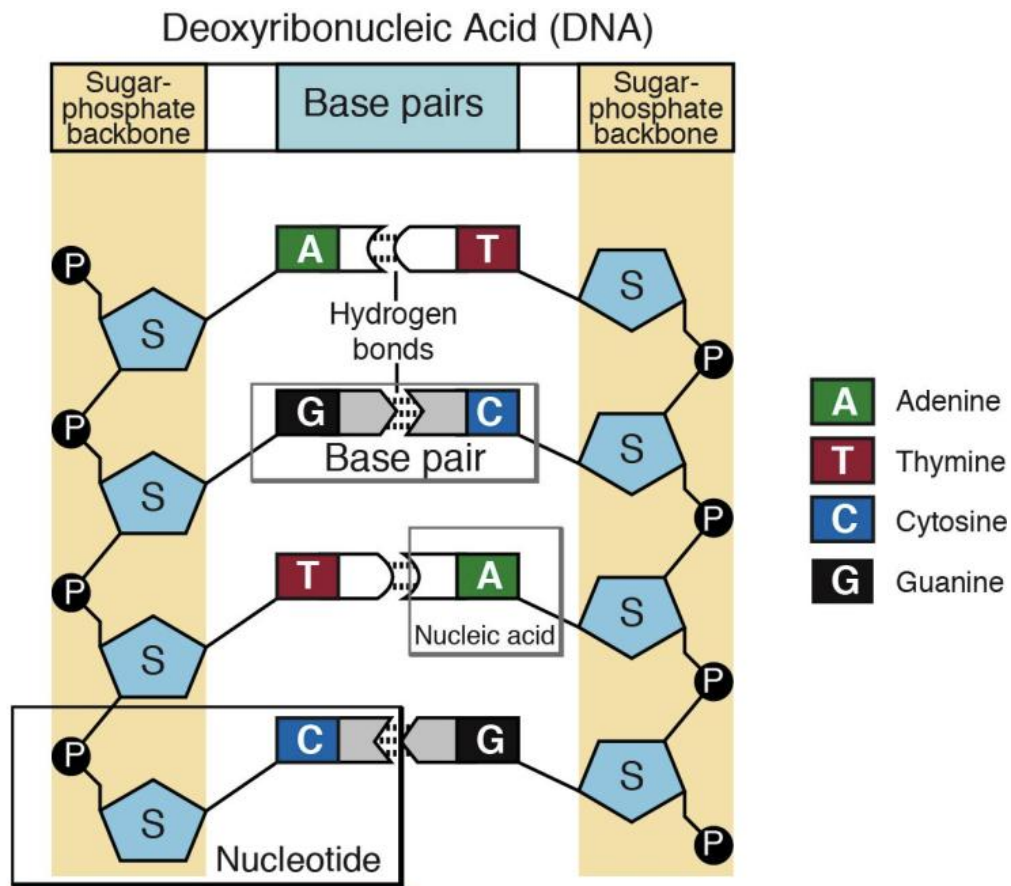
FIGURE 3.3: Double Helix Bondage
