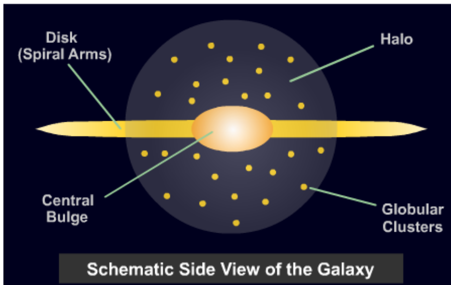
FIGURE 3.27: Three Basic Components of a Spiral Galaxy
