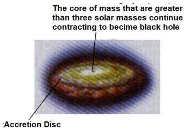
FIGURE 3.13: Formation of Black Hole
