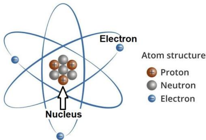
FIGURE 1.8: Atom
