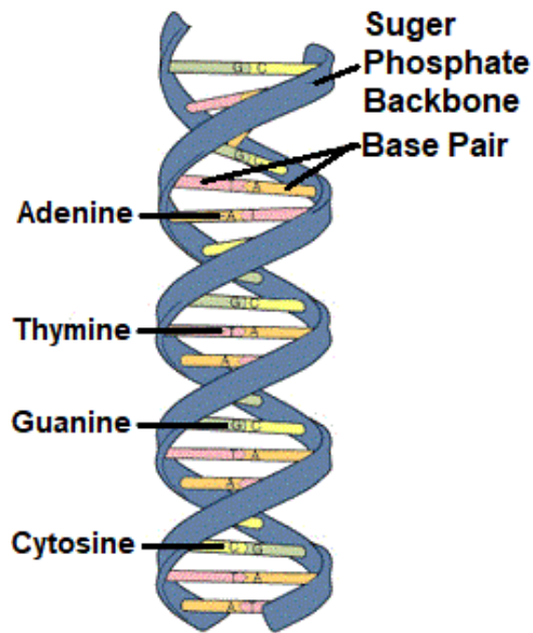
FIGURE.IGQ 2: Pair / DNA Double Helix Molecule
