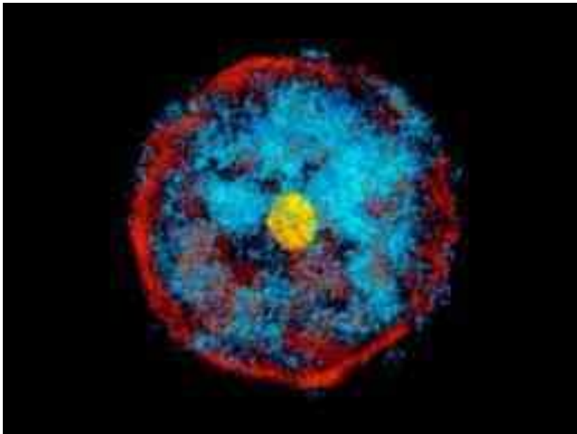
FIGURE 3.9: The Red Giant
