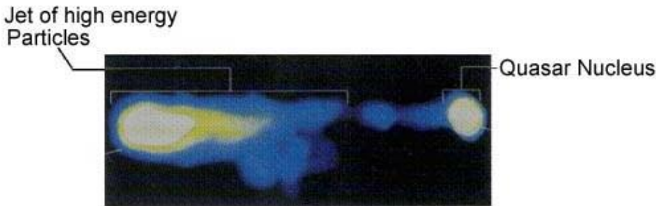
FIGURE 3.21: Quasar (3C273)
