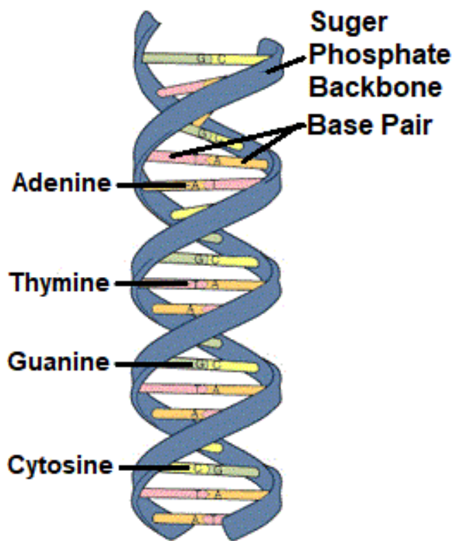
FIGURE 3.2: Pair / DNA Double Helix Molecule
