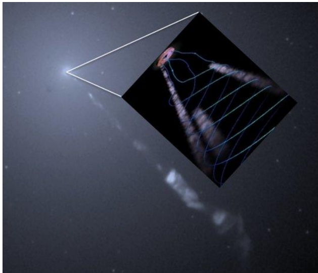
FIGURE 3.30: M87 jets from the Accretion Disk [Turbulent Mass Injection Process]
