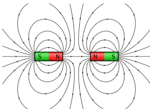
FIGURE 1.5: Magnetic Field
