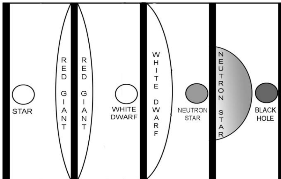
FIGURE 3.18: Stages of Collapsing Star
