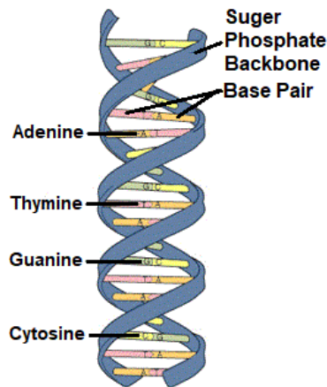
FIGURE 6.16: DNA Double Helix
