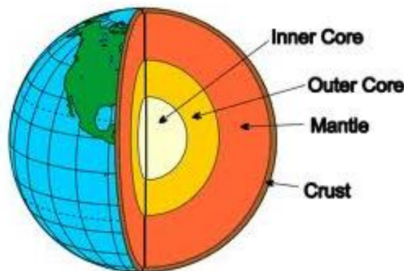
FIGURE 57.1: Earth's Interior
