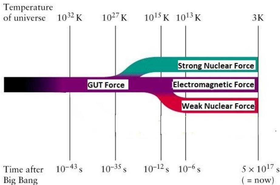
FIGURE 39.1: GUT Force
