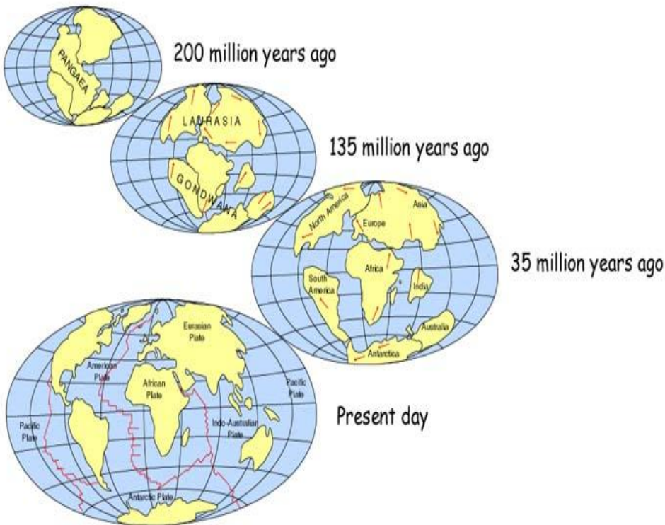
FIGURE 51.3: Drifting Continents
