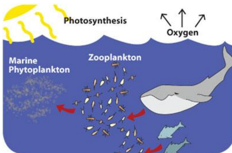
FIGURE 55.4: Mixed Layer
