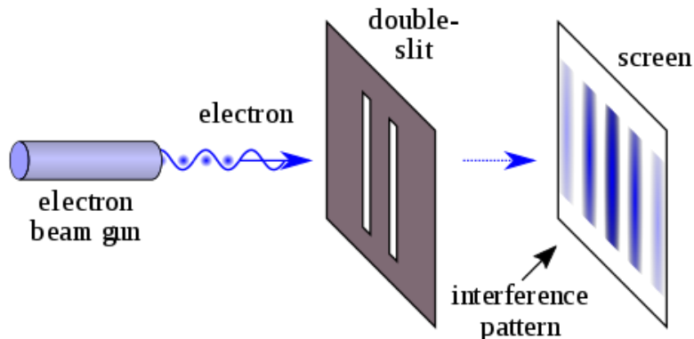
FIGURE 44.1: Wave-Particle Duality
