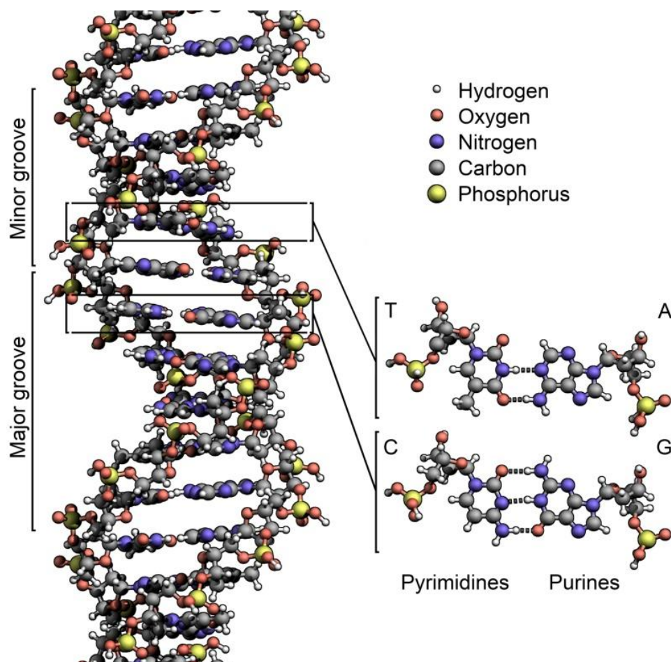
FIGURE 36.1: DNA Double Helix (Pairs)
