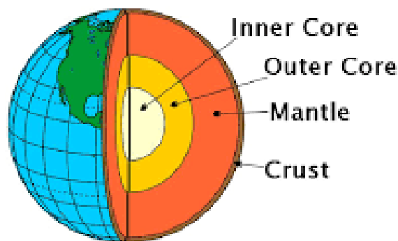
FIGURE 34.2: Earth's Interior
