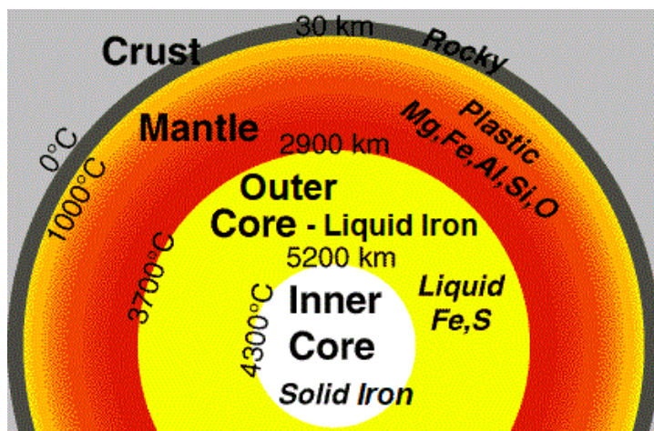
FIGURE 41.9: Earth's Interior
