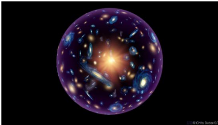
FIGURE 51.2: The Expansion
