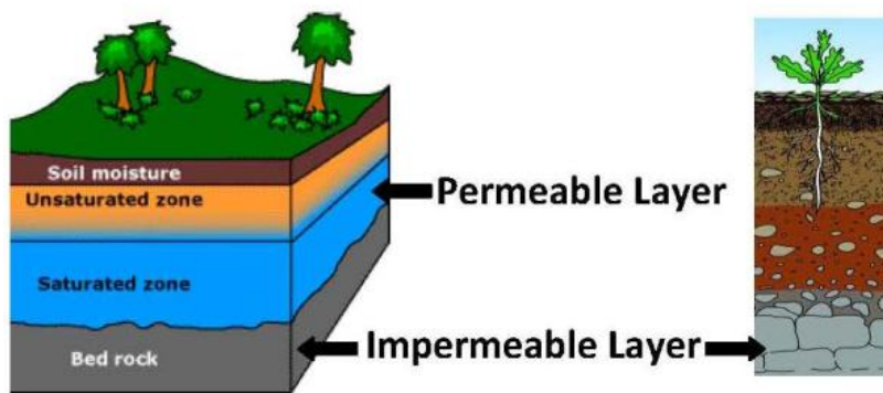
FIGURE 80.1: Ground Water
