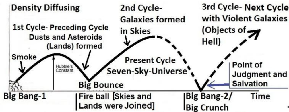
FIGURE 41.3: Cyclic Universe
