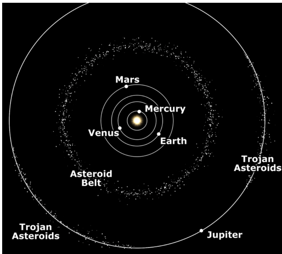
FIGURE 34.1: Asteroid Belt
