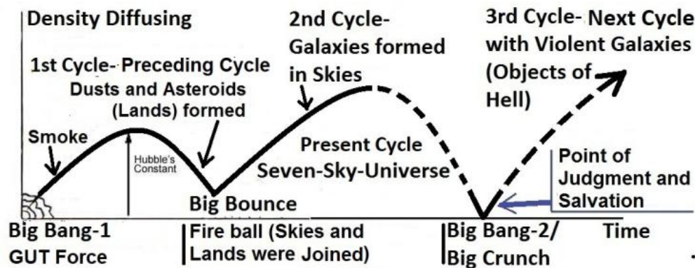
FIGURE 39.2: Cyclic Universe
