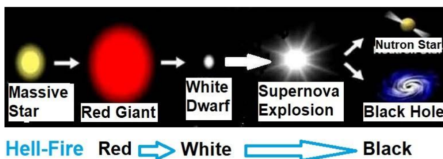
FIGURE 67.1: Stellar Evolution
