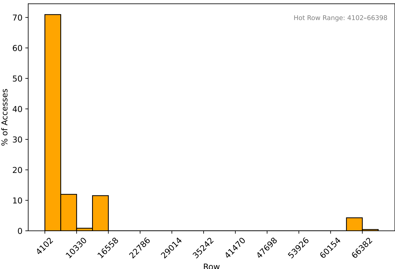
Row Access Distribution - C0R1B2
