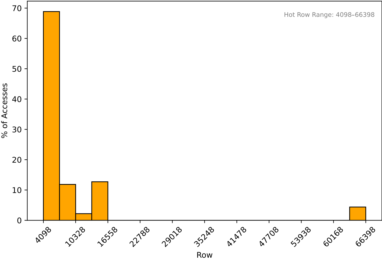
Row Access Distribution - C0R0B2
