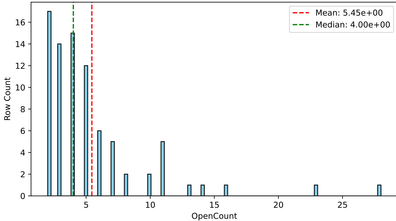
Histogram
