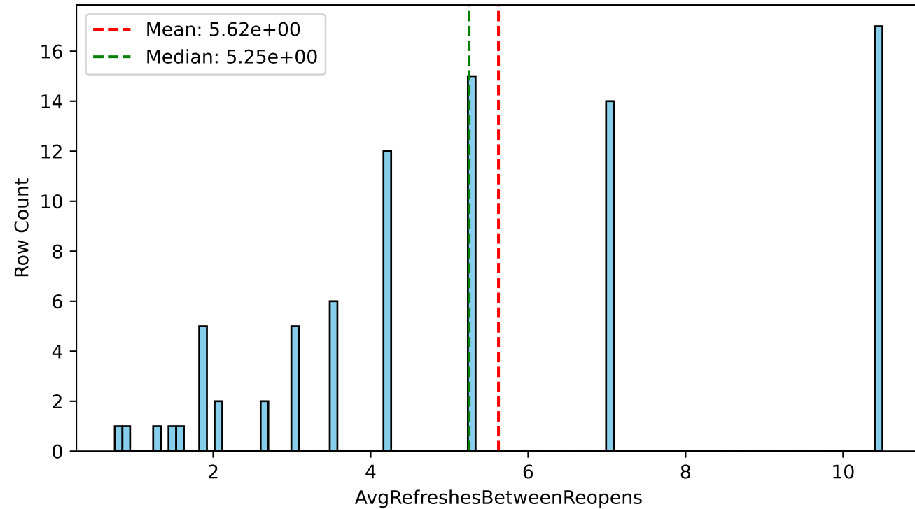
Histogram
