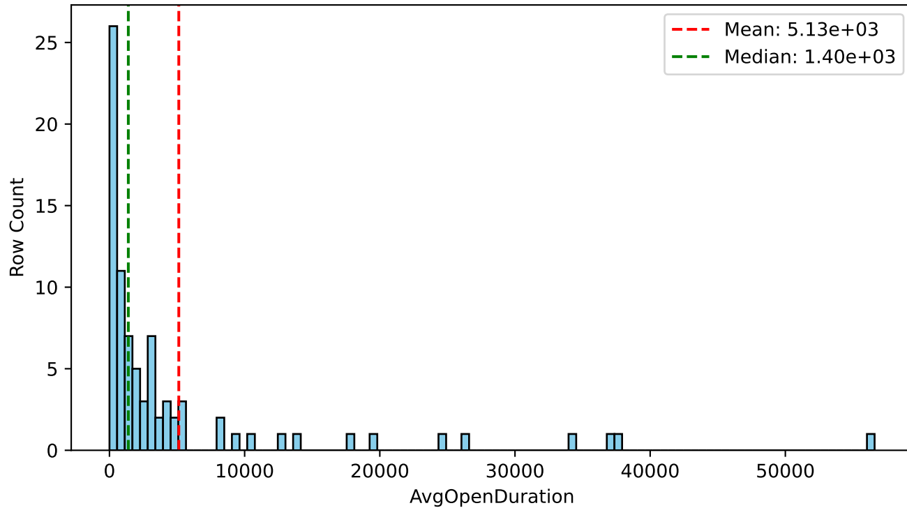
Histogram
