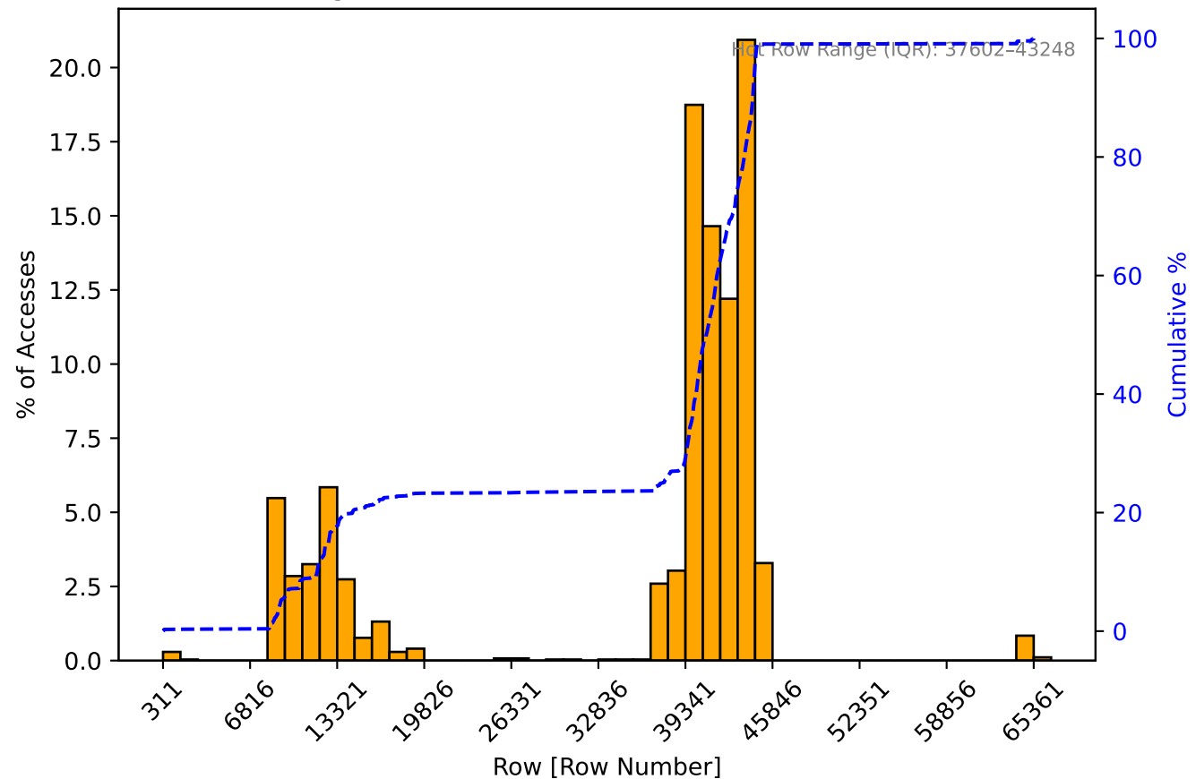
Merged Row Access Distribution - C0R0BG0B1
