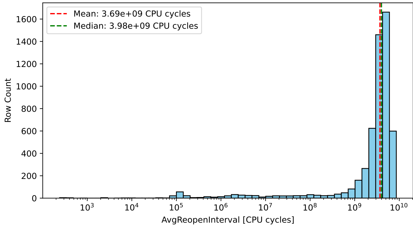
Histogram
