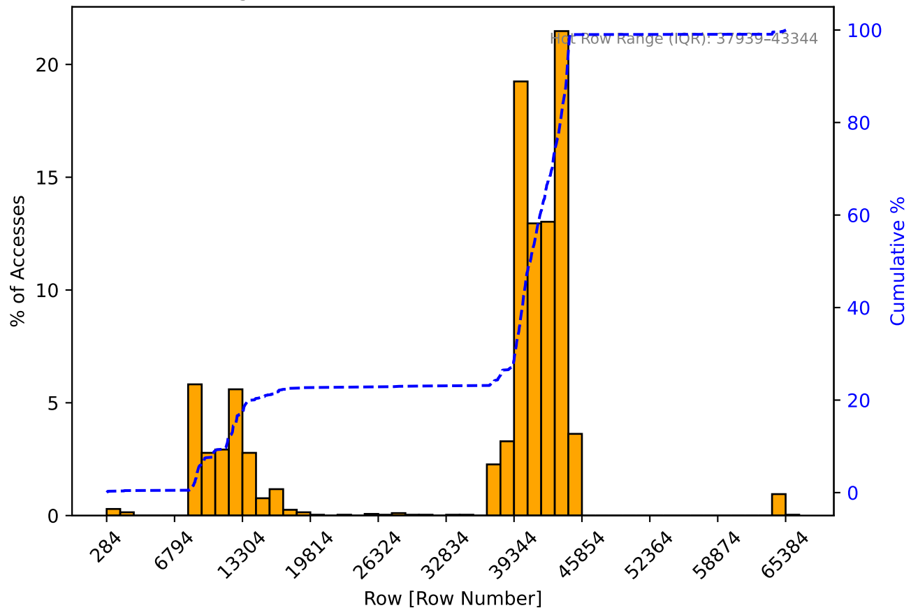
Merged Row Access Distribution - C0R0BG0B0
