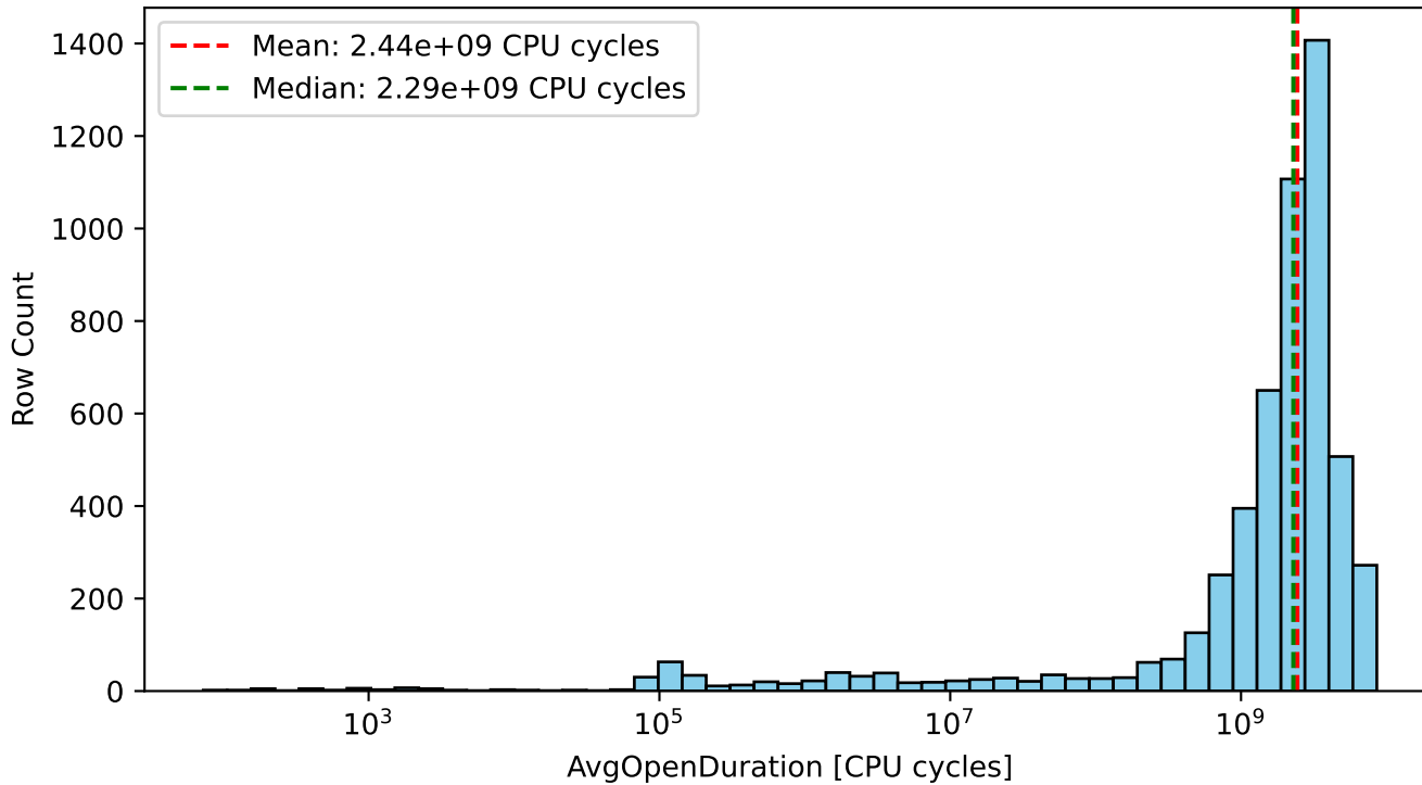
Histogram
