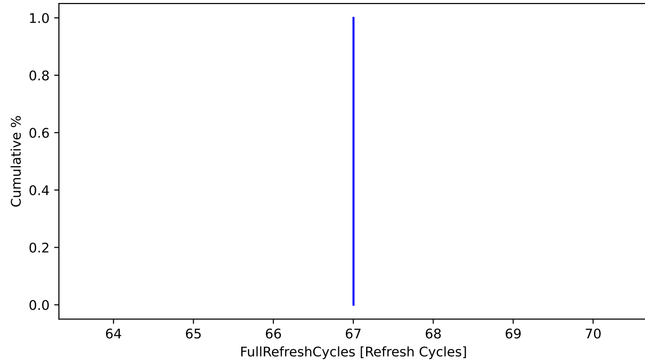
CDF
