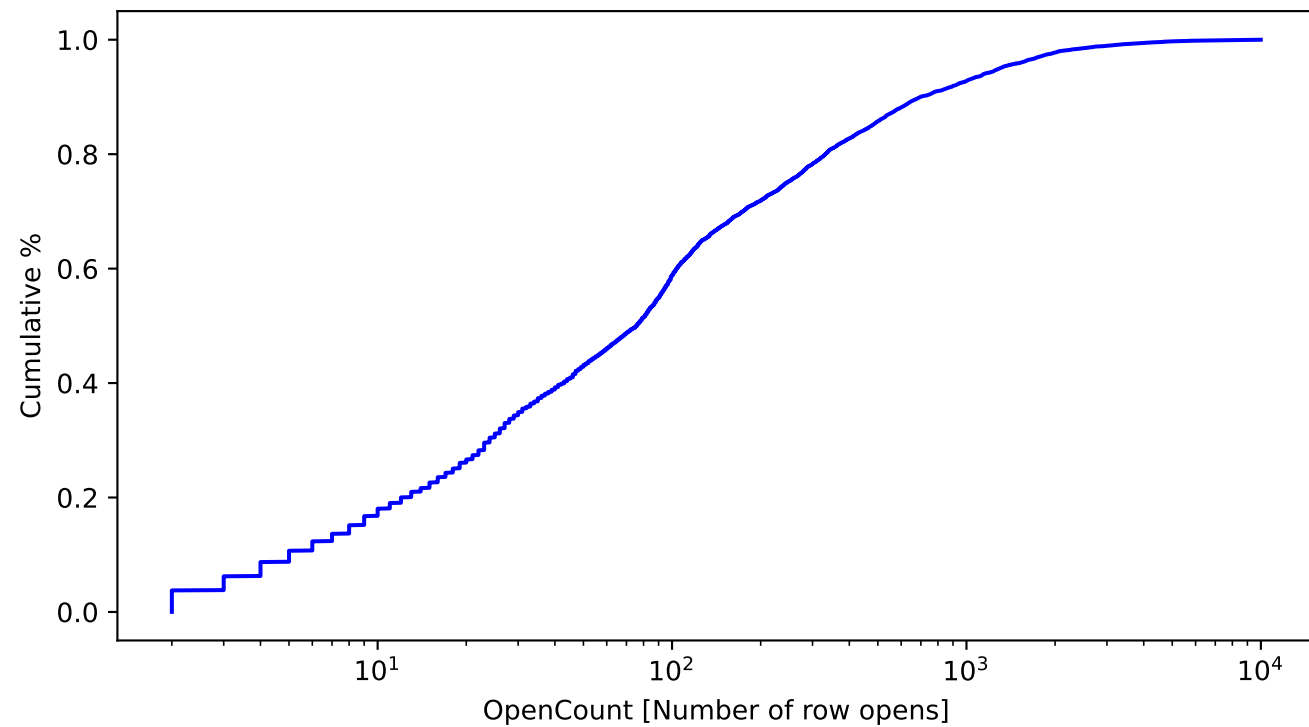
CDF
