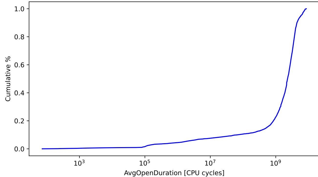
CDF
