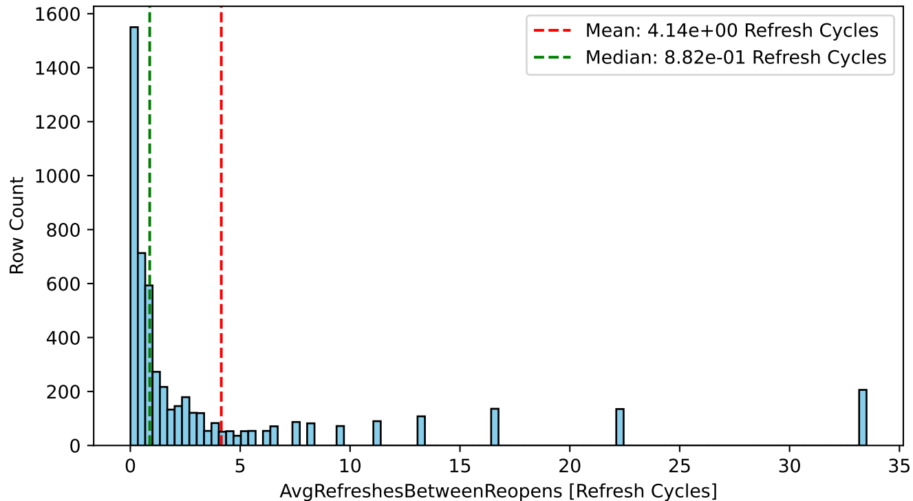
Histogram
