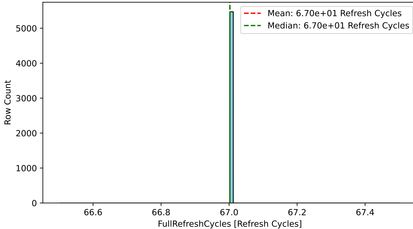
Histogram
