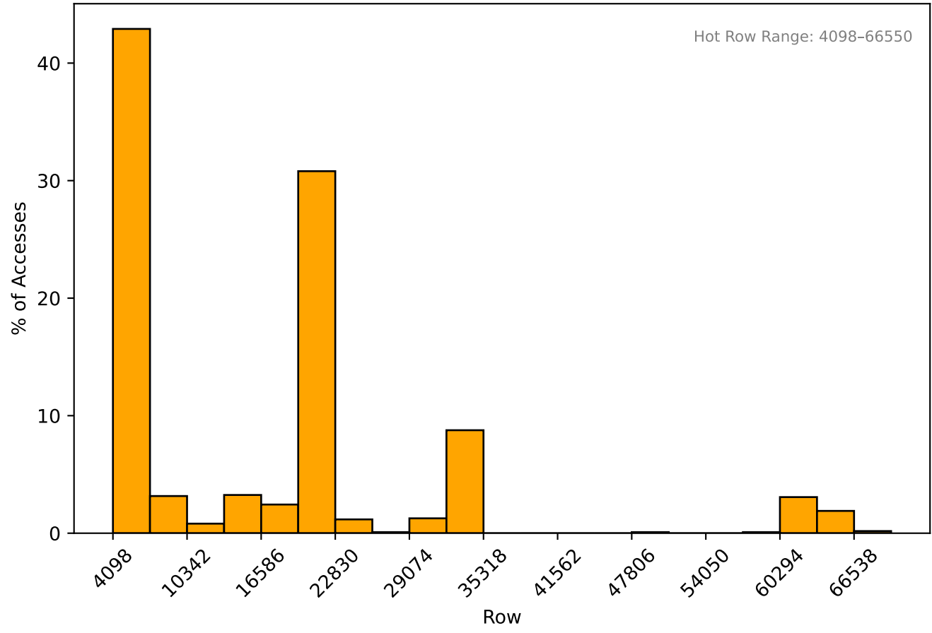
Row Access Distribution - C0R1B3
