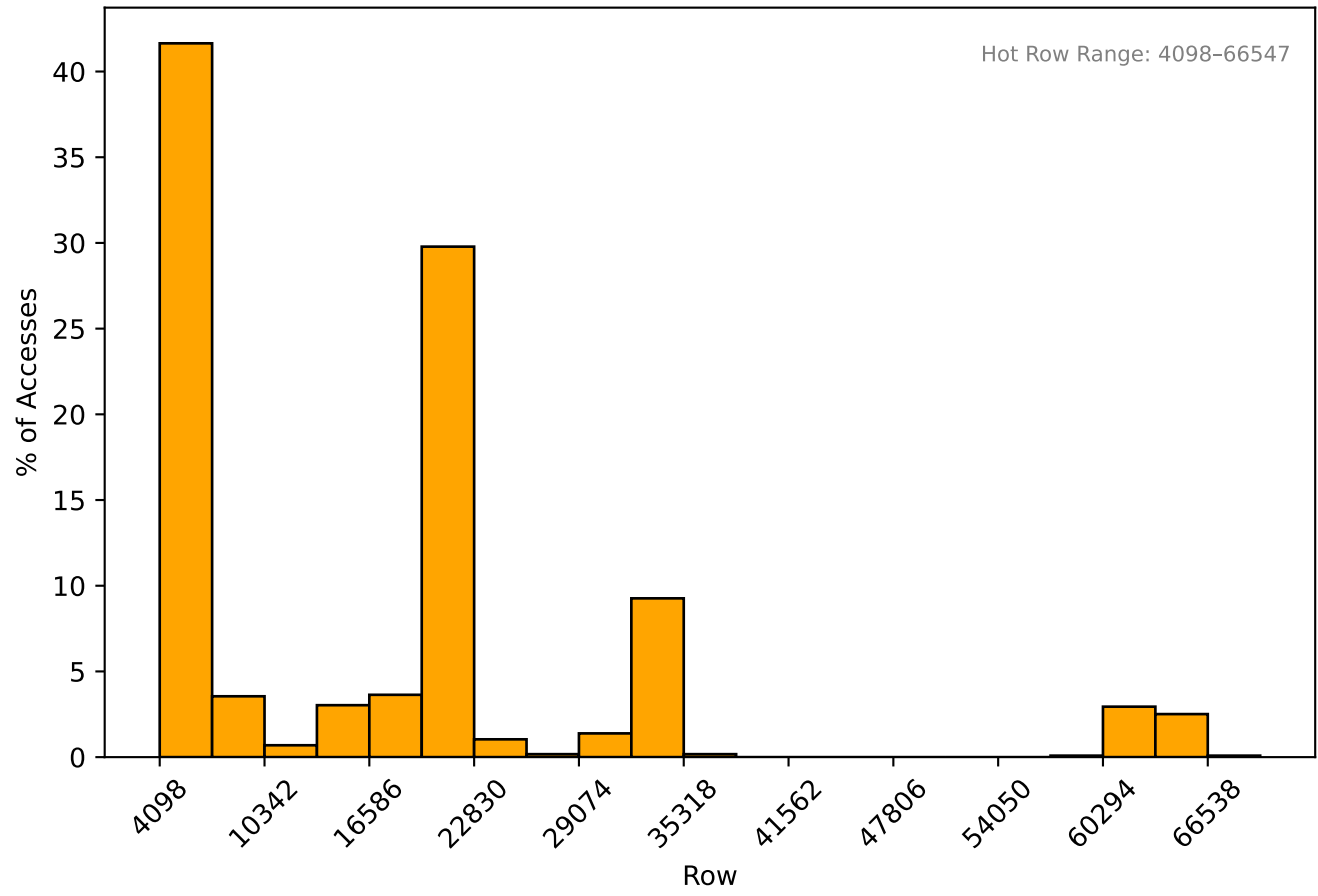
Row Access Distribution - C0R1B1
