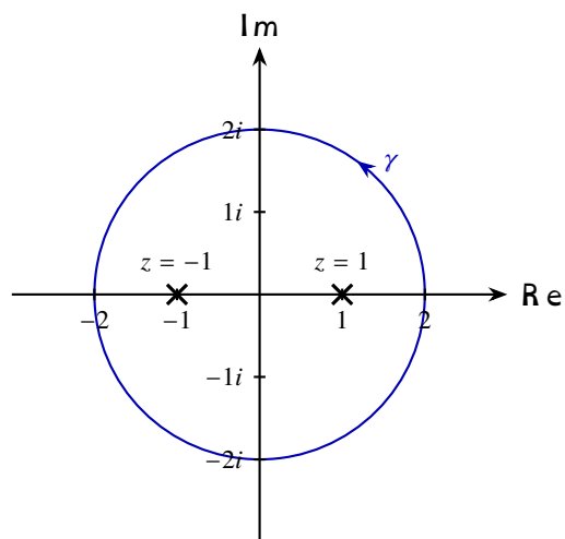
Figure 1: Positively oriented contour \gamma: |z| = 2 enclosing the poles of 1/(z^2 - 1) at z = \pm 1 (marked \times ).
