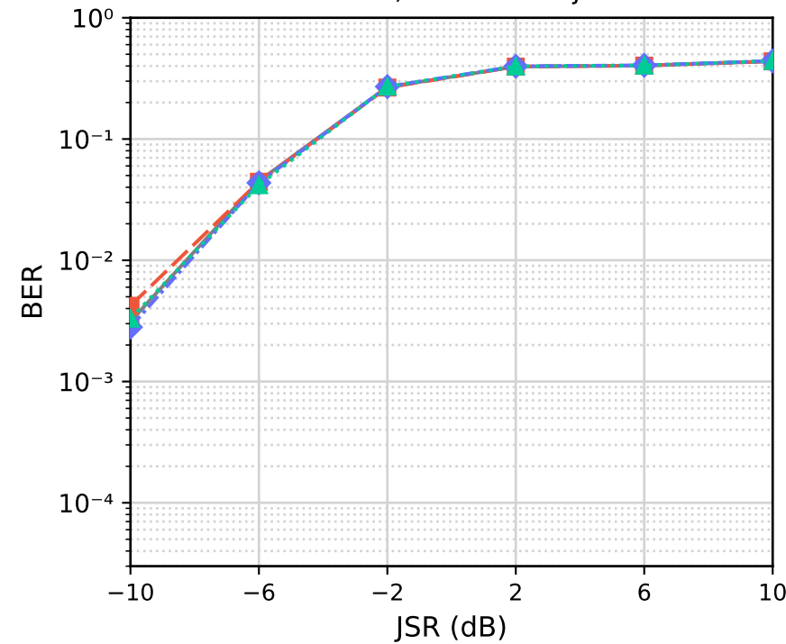
Fixed carrier, omniscient jammer
