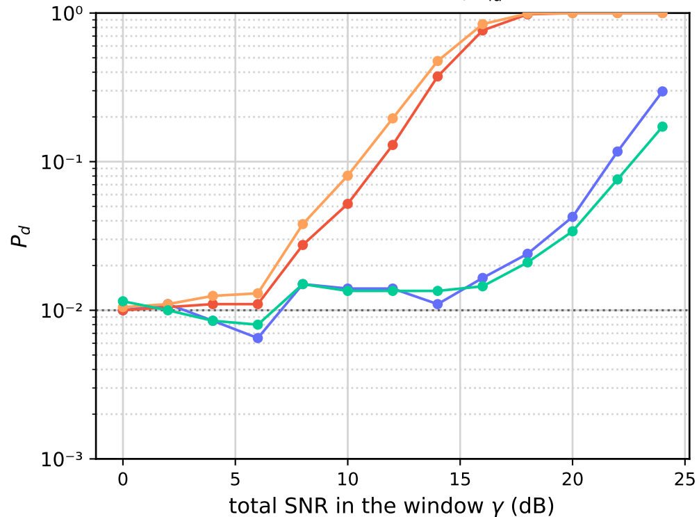
Channelized radiometer, P_{fa} = 10^{-2}
