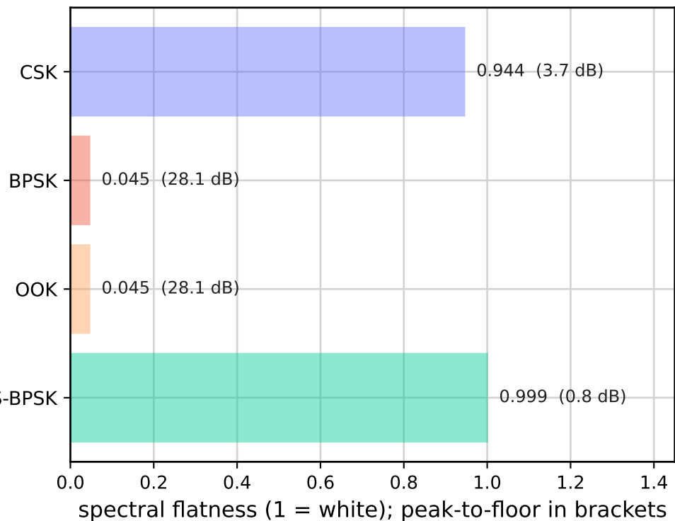
Spectral structure an interceptor can exploit
