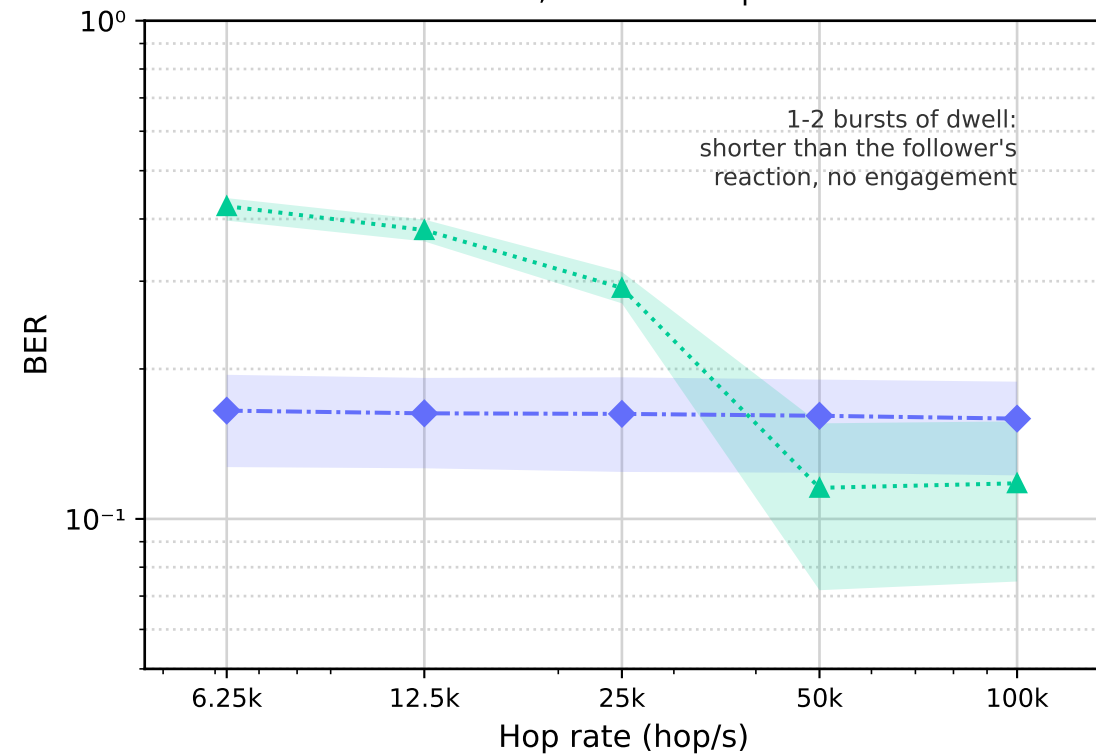
A tracker loses, a blind sweeper does not
