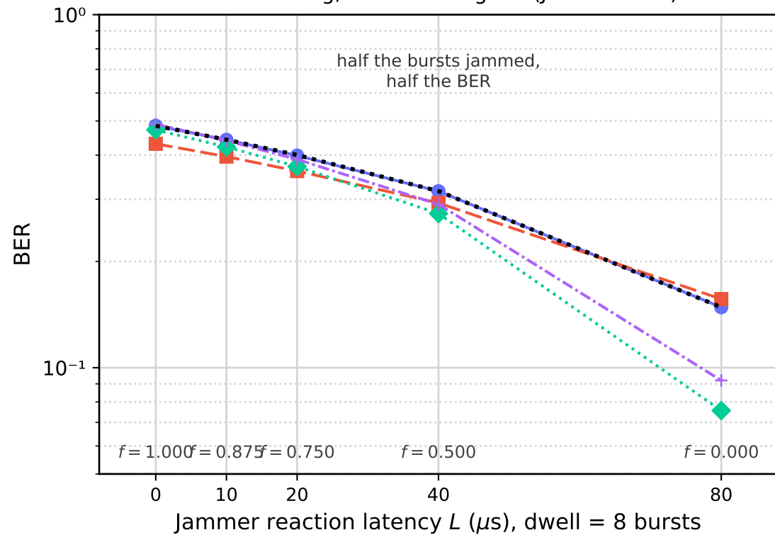
Time-sharing, not a soft regime (JSR = +6 dB)
