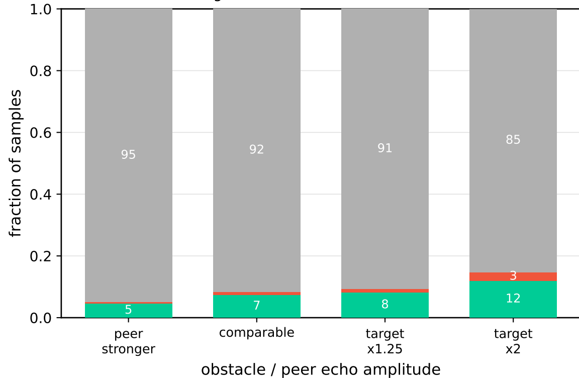
A stronger obstacle is identified more often
