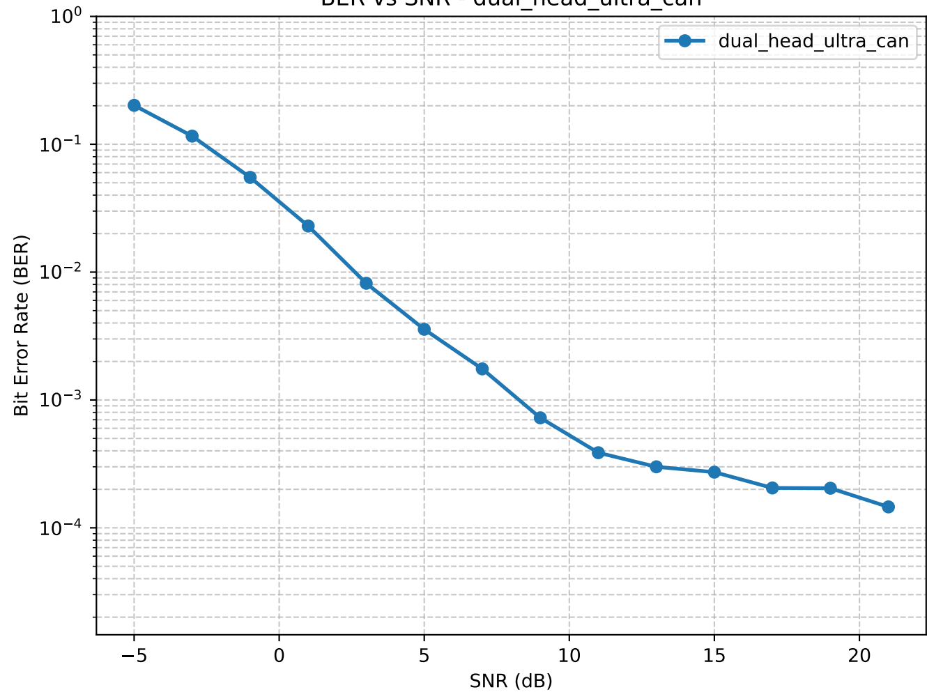
BER vs SNR - dual_head_ultra_can
