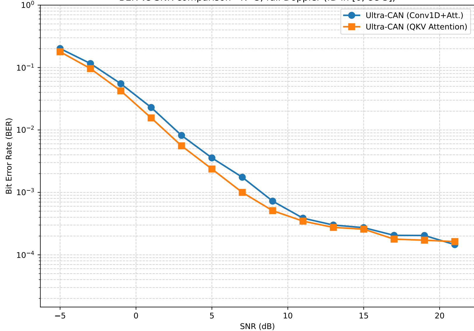
BER vs SNR comparison - K=3, full Doppler (fD in [0, 8e-5])
