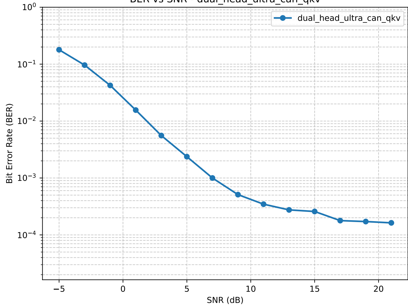
BER vs SNR - dual_head_ultra_can_qkv
