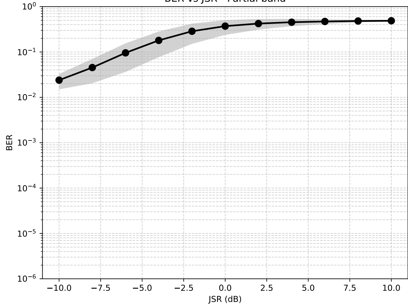
BER vs JSR - Partial band
