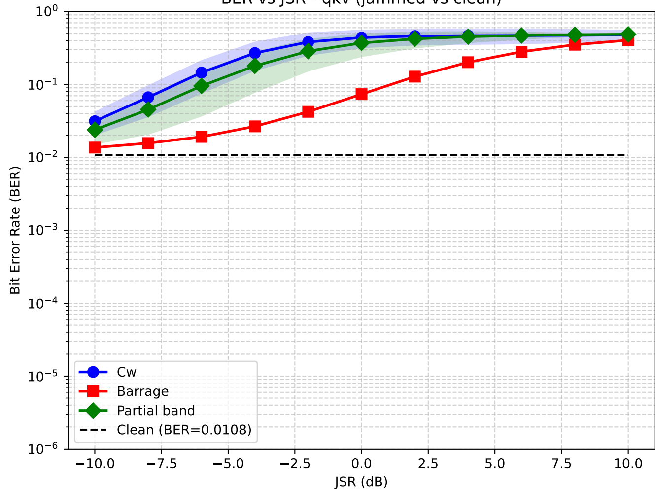
BER vs JSR - qkv (jammed vs clean)
