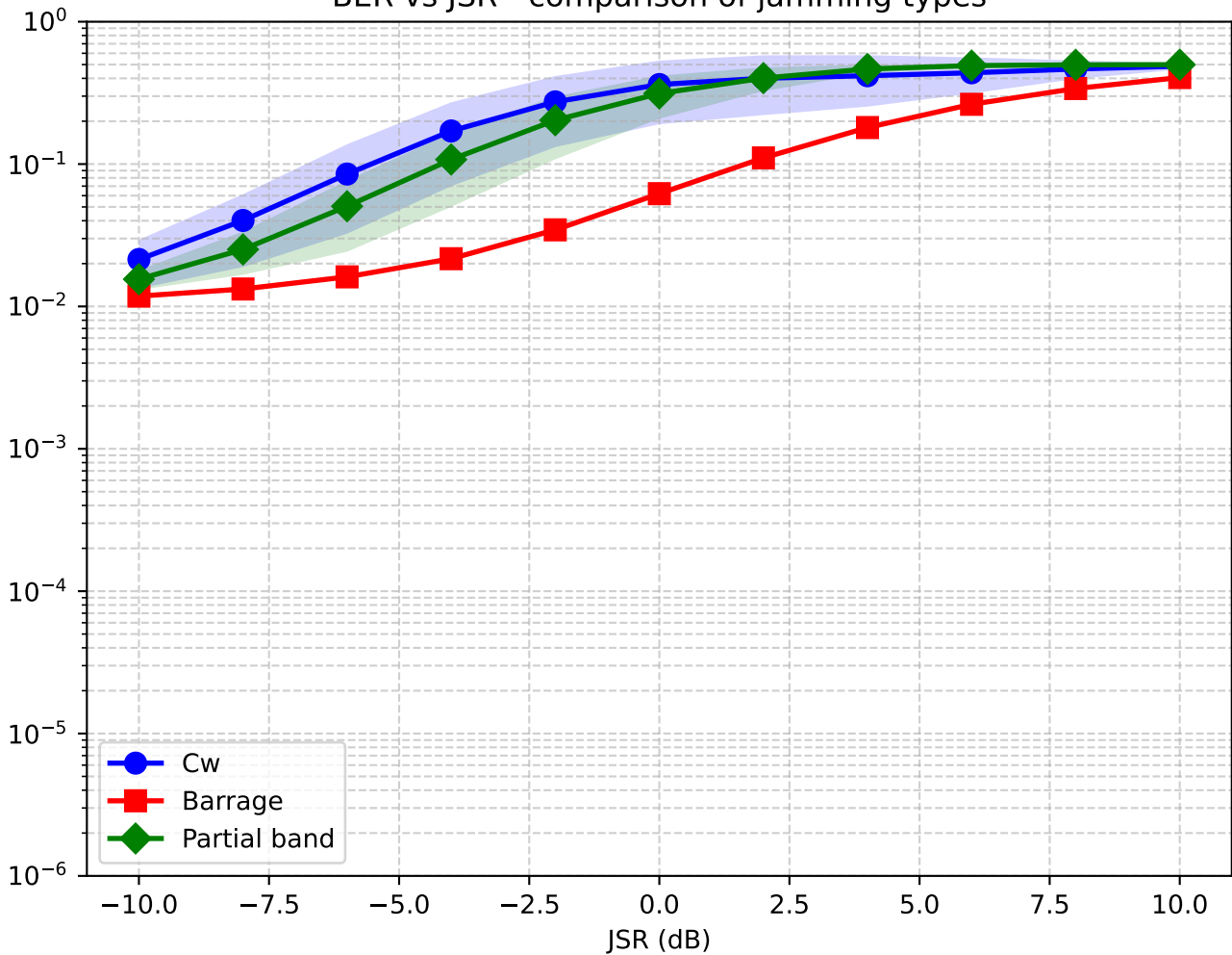
BER vs JSR - comparison of jamming types
