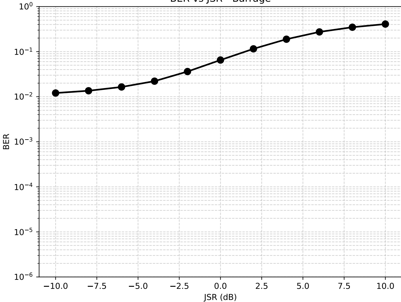
BER vs JSR - Barrage
