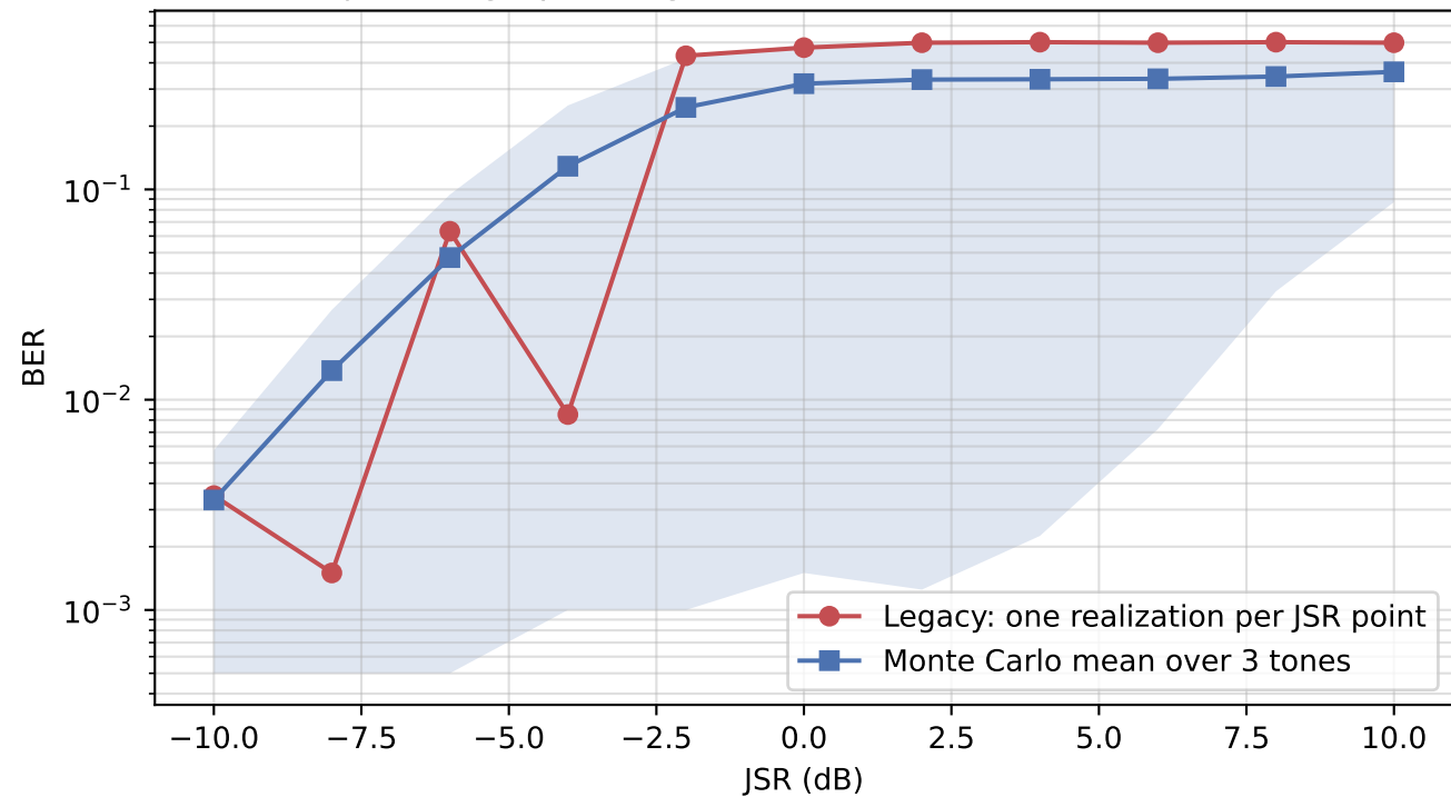
CW jamming, qkv: single-realization artifact vs Monte Carlo
