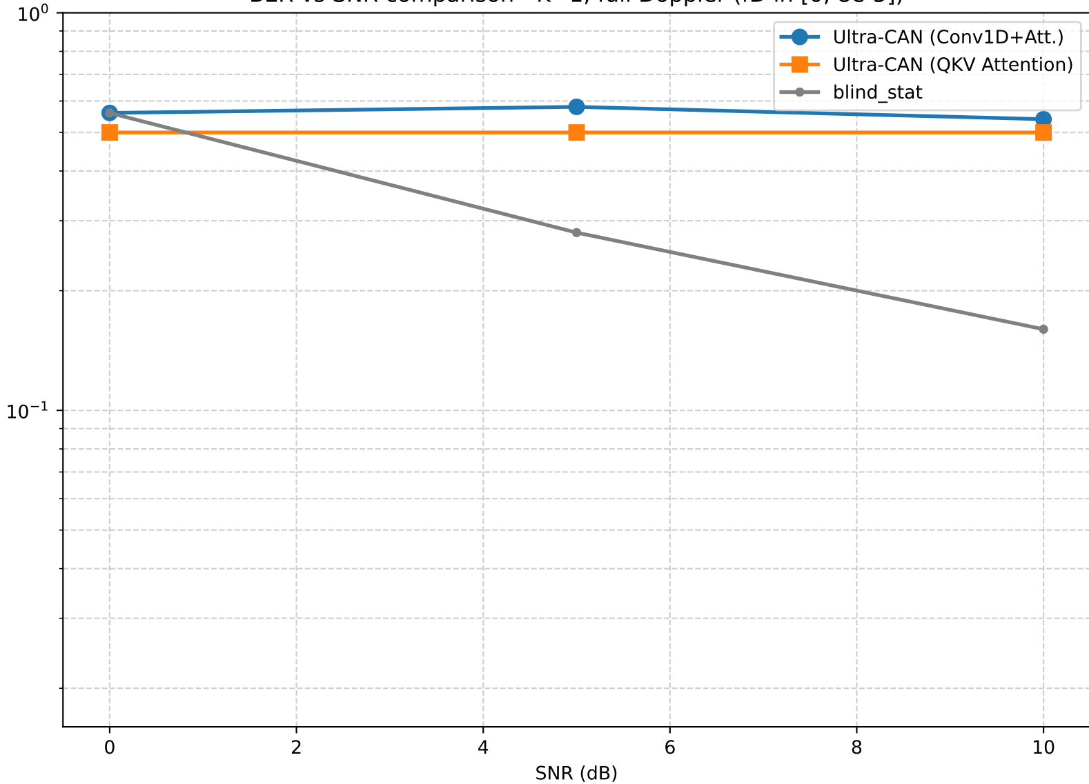
BER vs SNR comparison - K=1, full Doppler (fD in [0, 8e-5])
