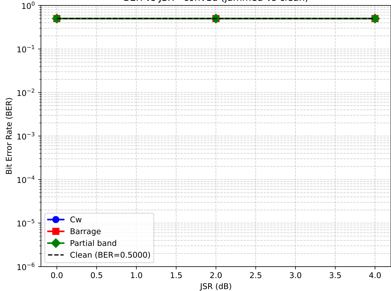
BER vs JSR - conv1d (jammed vs clean)
