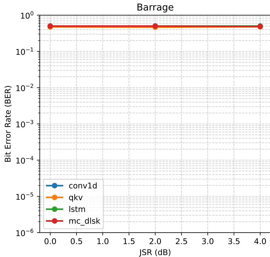
Jammed BER comparison - all models
