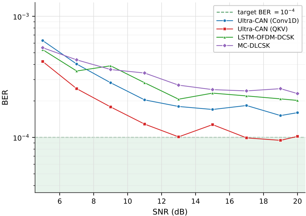
Multi-echo, low Doppler ( K = 3 )
