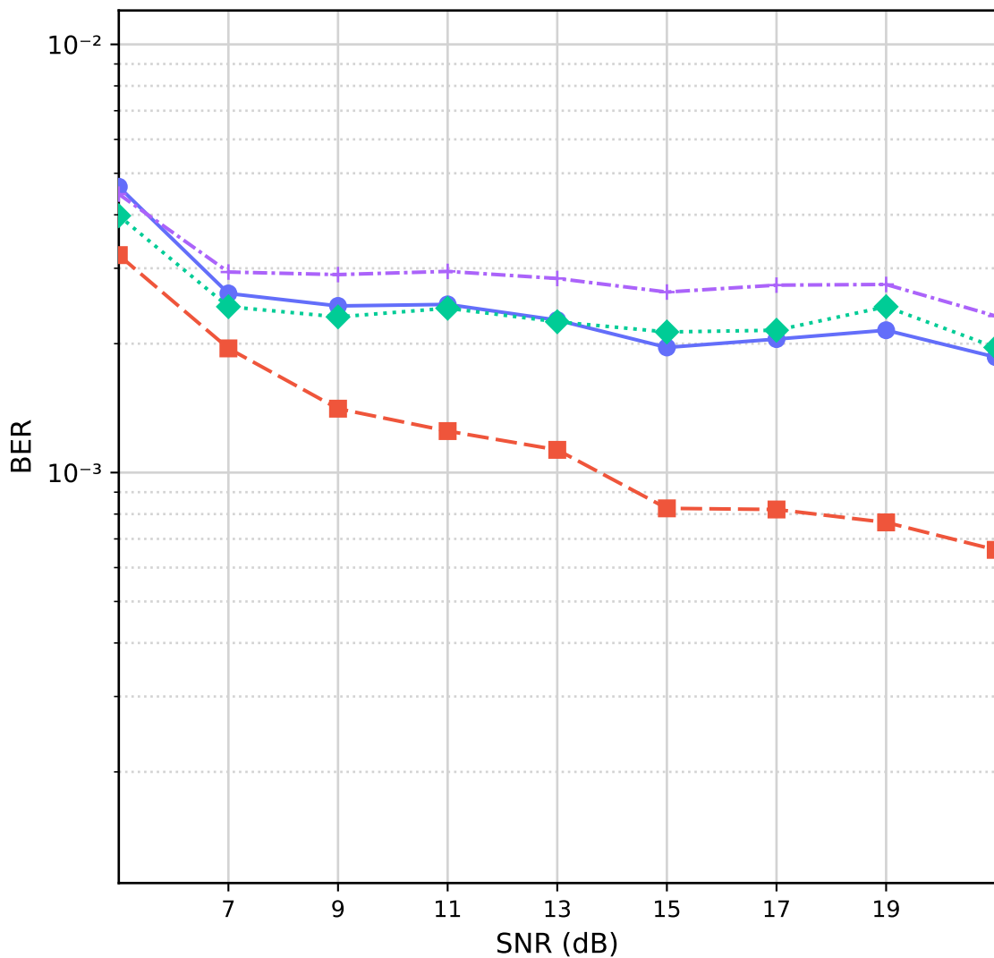
Multi-echo (K = 3)
