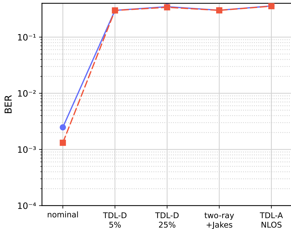
Communication: pooled BER
