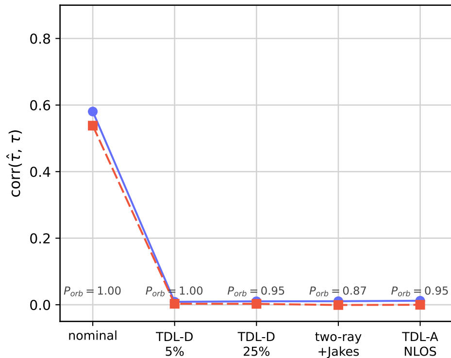
Sensing: delay correlation of the dominant echo
