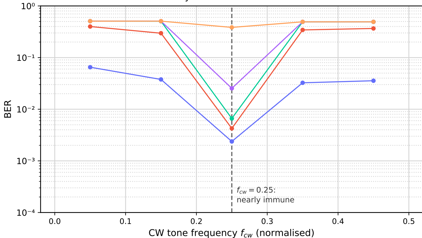
One tone in fifteen is nearly harmless: the CW curve needs a Monte Carlo
